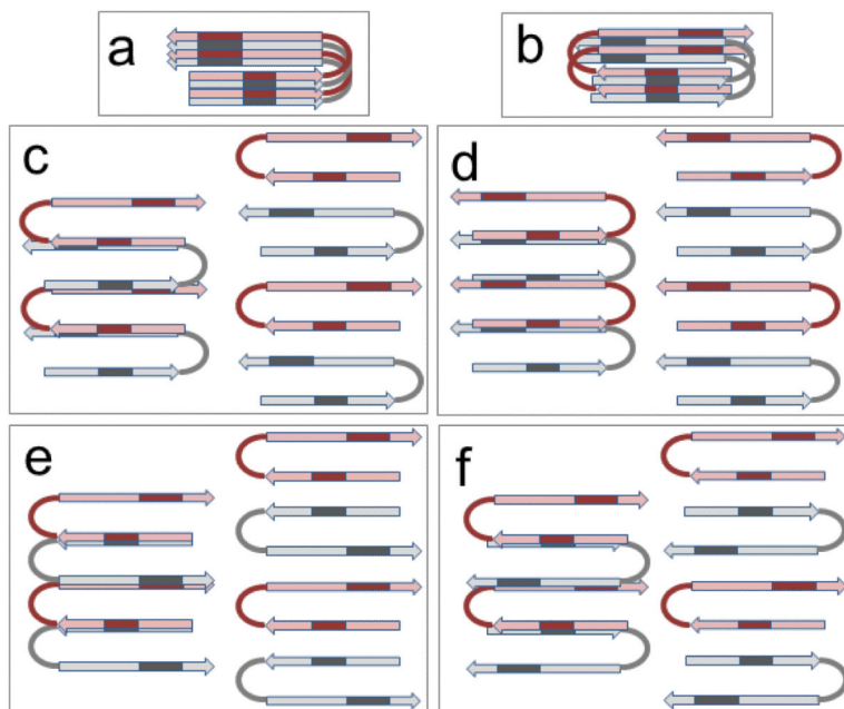
Figure 7. Schematic models for A \beta oligomerization through interactions between the core \beta -hairpin structures. Two arrows in each molecule represent two \beta -strands, connected by a loop or turn. The monomers are colored gray and pink, and the isotopically labeled segments are indicated by darker color. In all cases, the structures are stabilized by intramolecular H-bonding and intermolecular non-H-bonding contacts, i.e. ionic and/or hydrophobic interactions. The plane of the picture is parallel to the hairpin plane. In a) and b), the aggregation axis is perpendicular, and in c) to f) it is coplanar to the picture plane.
