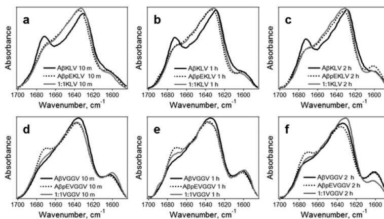
Figure 4. FTIR spectra of A\beta_{1-42} (black solid line), A\beta pE_{3-42} (dotted line), and their 1:1 combination (gray solid line) labeled either at K^{16}L^{17}V^{18} (a, b, c) or V^{36}G^{37}G^{38}V^{39} (d, e, f) in D_2O -based buffers of 50 mM NaCl, 50 mM Na,K-phosphate, pD 7.2, for 10 min (a,d), 1 h (b,e), and 2 h (c,f). Inset text in each panel intends to facilitate identification of spectra. For example, “ A\beta pEVGGV 1 h” means A\beta pE_{3-42} peptide labeled at V^{36}G^{37}G^{38}V^{39} incubated in buffer for 1 h. All spectra are normalized to a total area of 1.0.
