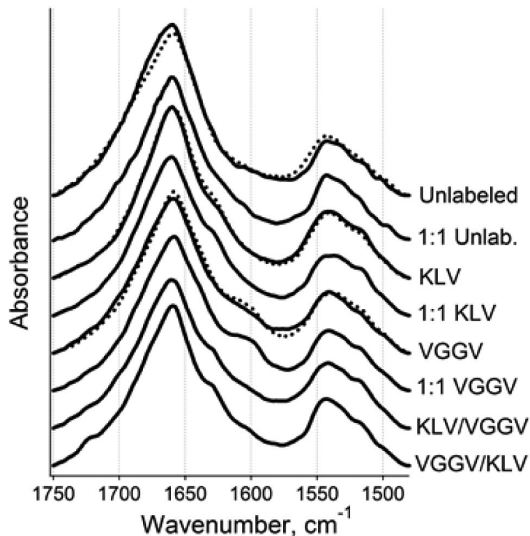
Figure 2. FTIR spectra of dry peptides in amide I and amide II regions. Spectra for unlabeled and isotopically labeled A\beta_{1-42} and A\beta pE_{3-42} peptides and their 1:1 combinations are presented. Dotted lines correspond to A\beta pE_{3-42} , and solid lines correspond either to A\beta_{1-42} or to combined samples, as indicated. KLV or VGGV imply the peptides have been labeled at K^{16}L^{17}V^{18} or V^{36}G^{37}G^{38}V^{39} , respectively. In KLV/VGGV or VGGV/KLV samples, the first stretch applies to A\beta_{1-42} and the second to A\beta pE_{3-42} . All spectra are normalized to a total area of 1.0.
