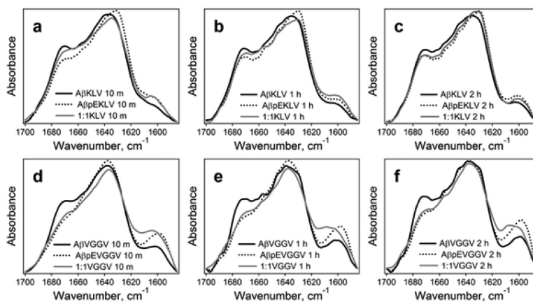
Figure 5. FTIR spectra of A\beta_{1-42} (black solid line), A\beta_{pE3-42} (dotted line), and their 1:1 combination (gray solid line) labeled either at K^{16}L^{17}V^{18} (a, b, c) or V^{36}G^{37}G^{38}V^{39} (d, e, f) in D_2O -based buffers of 10 mM Na,K-phosphate, pD 7.2, for 10 min (a,d), 1 h (b,e), and 2 h (c,f). Inset text is explained under Figure 4. All spectra are normalized to a total area of 1.0.
