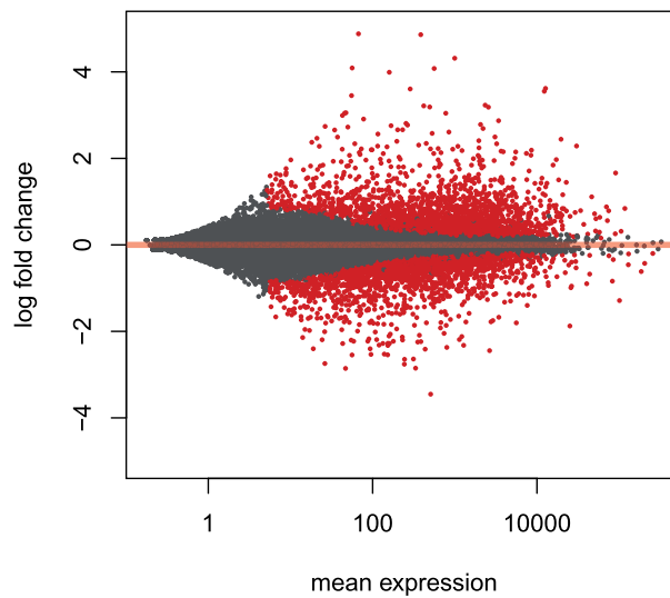
Figure 10. An MA-plot of changes induced by treatment. The log2 fold change for a particular comparison is plotted on the y-axis and the average of the counts normalized by size factor is shown on the x-axis ("M" for minus, because a log ratio is equal to log minus log, and "A" for average). Each gene is represented with a dot. Genes with an adjusted p value below a threshold (here 0.1, the default) are shown in red.
