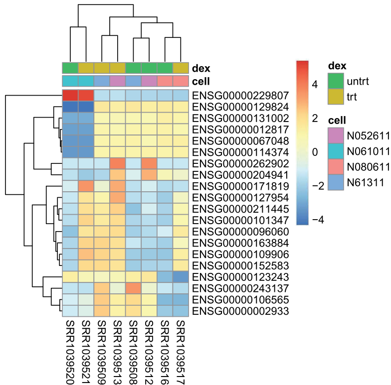
Figure 13. Heatmap of relative rlog -transformed values across samples. Treatment status and cell line information are shown with colored bars at the top of the heatmap. Note that a set of genes at the top of the heatmap are separating the N061011 cell line from the others. In the center of the heatmap, we see a set of genes for which the dexamethasone treated samples have higher gene expression.
