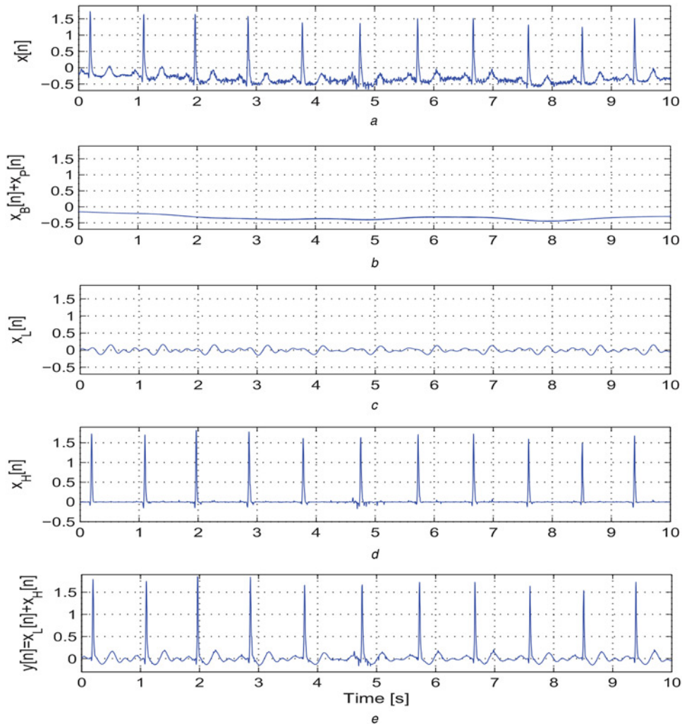
Fig. 2 Outputs of the proposed sparse decomposition approach a Original ECG signal taken from a mitbaha record 101 containing narrow QRS complexes, BW, and background noises b Extracted BW x_{\text{B}}[n] plus PLI signal x_{\text{P}}[n] c Extracted LF signal x_{\text{L}}[n] including the P-wave, LF components of QRS complex, and T-wave d Extracted HF x_{\text{H}}[n] including the high-slope portions of QRS complex and spike components e Filtered signal y[n] = x_{\text{L}}[n] + x_{\text{H}}[n] after discarding the x_{\text{B}}[n] and x_{\text{P}}[n]
