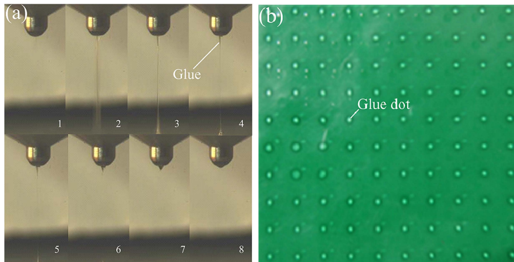
Figure 11. Dot forming process from (a) and jetting dot matrix from (b).
