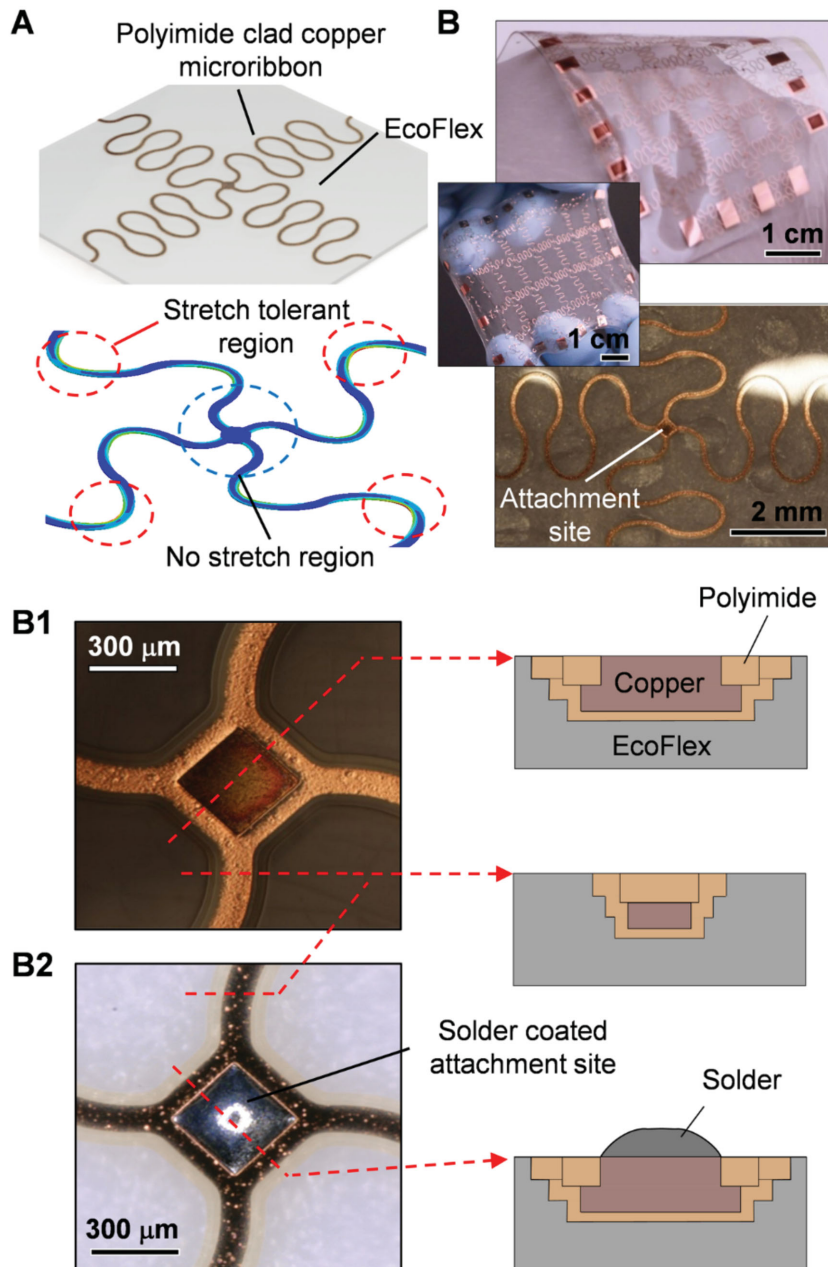
Figure 2. Schematics (A) and photographs (B) of the fabricated stretchable bottom electrode. The structure is designed to be compatible with a fluidic self-assembly process that requires the integration of a solder bump in a no-stretch-assembly region. One stress profile calculation (also being discussed in Figure 3) is shown. The profile depicts a no-stretch-region (blue circle). The no-stretch-region is the preferred location to define an attachment site for the LEDs with minimal mechanical stress. The attachment sites within the array are electrically connected using 100 \mu\text{m} wide and 5 \mu\text{m} thick meander shaped copper traces. These traces are mechanically and chemically stabilized using a polyimide cladding with the illustrated cross-sections. The color difference in the corresponding top view photographs is due to a difference in the background; a white paper cloth versus a transparent background.
