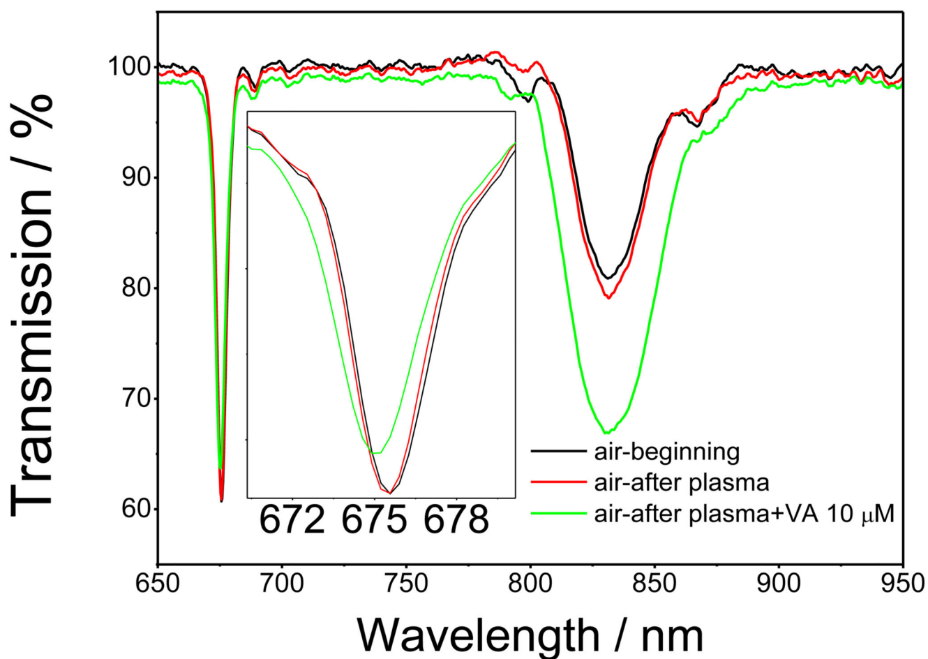
Figure 4. TS of the nano-MIP coated LPG, measured in air before (black line) and after exposure to, porcine plasma (red line) and porcine plasma spiked with 10 \mu M of VA (green line)
