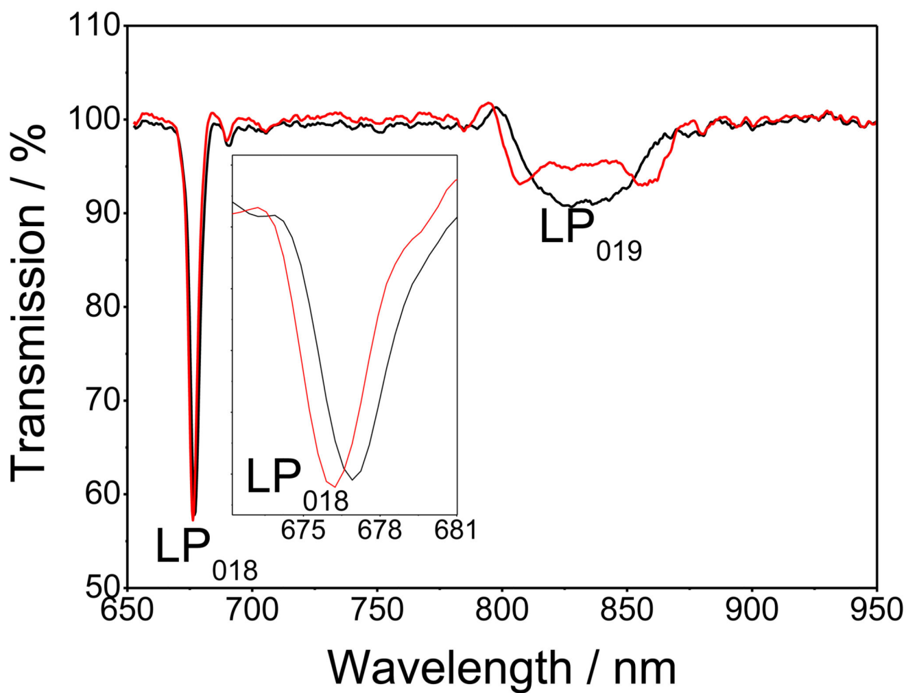
Figure 1. TS of the LPG measured in air: black line, before APTMS deposition, and red line, after APTMS deposition
