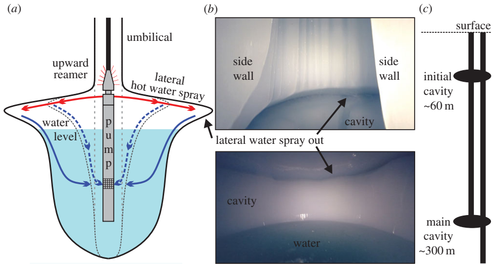
Figure 3. (a) Schematic of cavity formation, (b) images from inside a cavity at 90 m depth and (c) schematic of the proposed two-hole, two cavity system.
