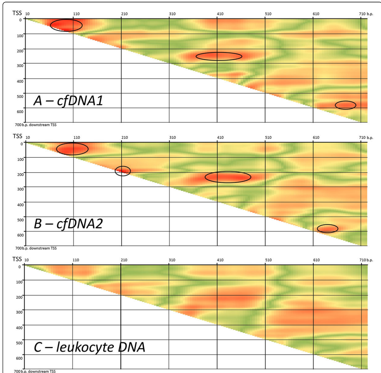
Figure 7 Overview of statistically significant areas in the TSS downstream region. Pictures A, B and C represents the results for the cfDNA sample 1, cfDNA sample 2 and first patient's leukocyte DNA respectively. Black circles points out combinations of positions which give statistically significant ( p -value < 0.05) separation of tissue specific and widely expressed genes.
