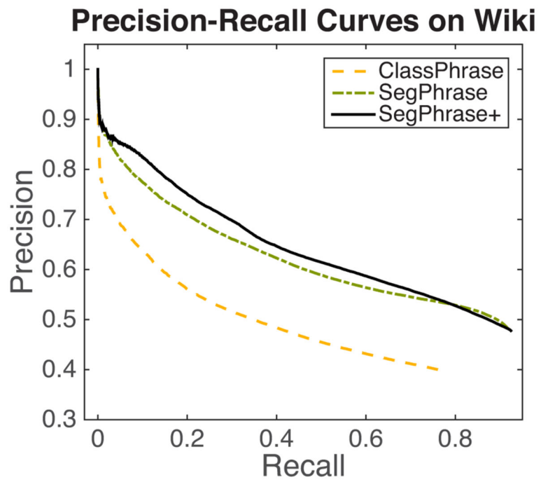
Figure 6. Precision-recall curves of the 3 proposed methods tested on Wikipedia dataset
