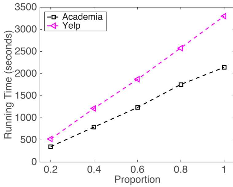
Figure 3. Runtime on different proportions of data
