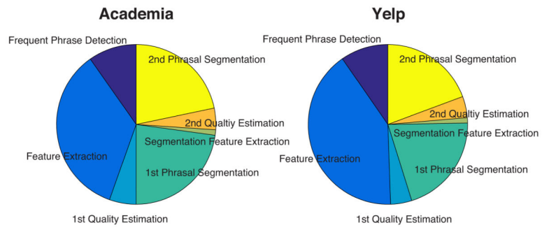
Figure 4. Runtime of different modules in our framework on Academia and Yelp dataset
