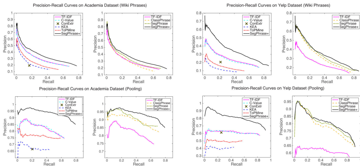
Figure 1. Precision-recall in 4 groups of experiments: (Academia, Yelp) × (Wiki phrase, pooling). Within each group, two figures are shown on par: the left compares SegPhrase+ with existing methods, and the right compares among the 3 proposed methods in this paper together with TF-IDF baseline
