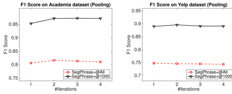
Figure 5. Performance variations of SegPhrase+ and ClassPhrase+ with increasing iterations
