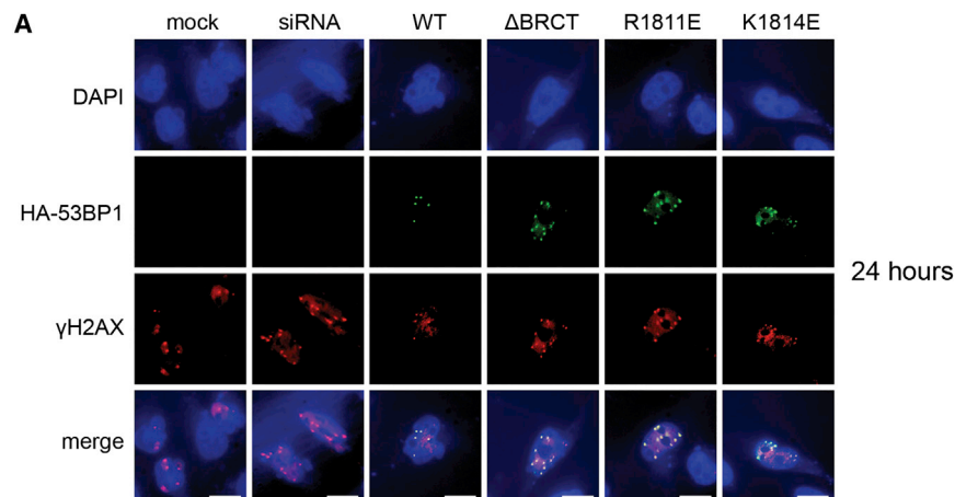
Figure 4. Slow Repair of Damage in Heterochromatin Is Defective in 53BP1-BRCT 2 Phospho-Binding Mutants
