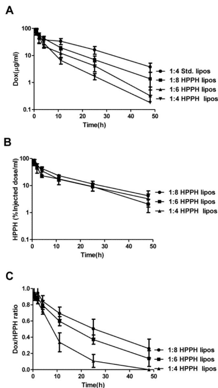
Figure 3. Blood circulation of liposomes with different drug-to-lipid loading ratios (A) Amount of Dox in blood of mice injected with HPPH liposomes or Std. liposomes at the indicated D:L molar ratio at a Dox dose of 5 \text{ mg kg}^{-1} ; (B) % of injected HPPH dose in 1ml blood for the same mice used in A. (C) Dox-to-HPPH ratio (% injected dose ratio) for the same mice used in A. Results are mean \pm std. dev. for n=4 mice.
