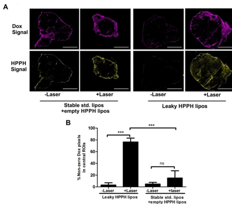
Figure 5. Dox and HPPH-lipid distribution 24 hours after treatment with or without laser irradiation
