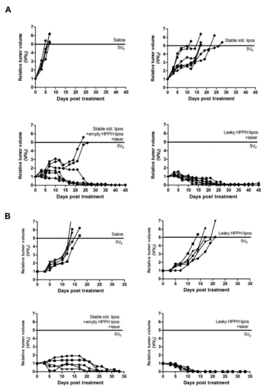
Figure 6. Complete and rapid tumor eradication with a single phototreatment using Dox-loaded HPPH liposomes
