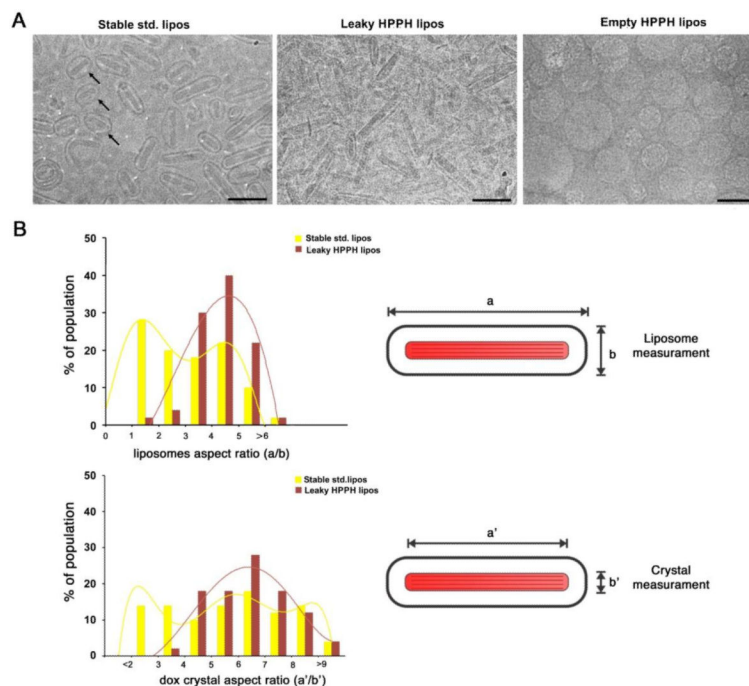
Figure 2. Morphology of Dox-loaded stable standard and leaky HPPH liposomes with a 1:4 drug- to-lipid ratio
