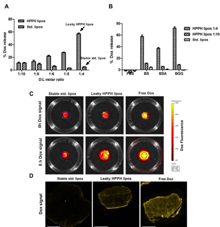
Figure 1. Controlling Dox release from HPPH liposomes by tuning the drug to lipid ratio (A) Dox release from HPPH or std. liposomes in 50% bovine serum following 24 hours incubation at 37 °C at the indicated drug-to-lipid (D:L) molar ratios. Mean \pm S.D. for n=3. (B) Dox release in PBS, 50 mg/mL bovine serum albumin (BSA), 50% bovine serum (BS) or 25 mg/ml bovine gamma globulin (BGG) following 24 hours incubation at 37 °C with indicated liposomes. Mean \pm S.D. for n=3. (C) Permeation of Dox from liposomes pre-incubated with serum in an acrylamide gel. Site of initial incubation is marked by a circle. The upper panel shows the initial Dox distribution while lower panel shows Dox fluorescence 6 hours later. Dox signal in leaky HPPH liposomes group is higher than stable std. liposomes due to unquenching of Dox following release from the liposomes. (D) Dox permeation into tumors ex-vivo. Dox fluorescence is shown for whole MIA Paca-2 tumor micrographs. Tumors were incubated with leaky HPPH liposomes or stable std. liposomes in whole bovine serum for 24 hours. Due to the destabilization by serum proteins, Dox from leaky HPPH liposomes penetrated further and reached the center of the tumors, resulting in more homogeneous distribution of Dox in the tumor. A 3 mm scale bar is shown. Representative images for n=3.
