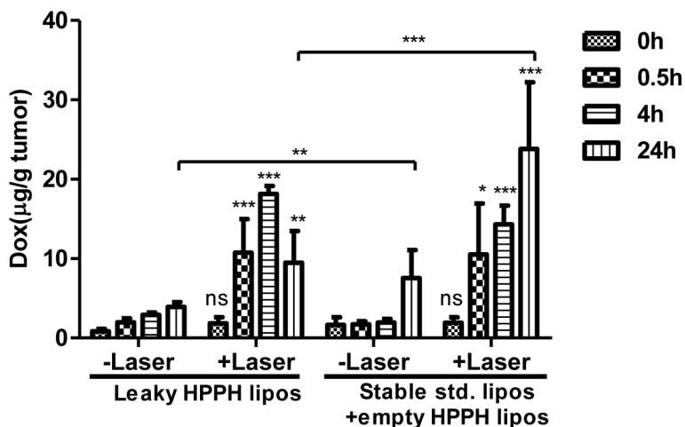
Figure 4. PDT-induced enhanced Dox deposition in a dual tumor model
