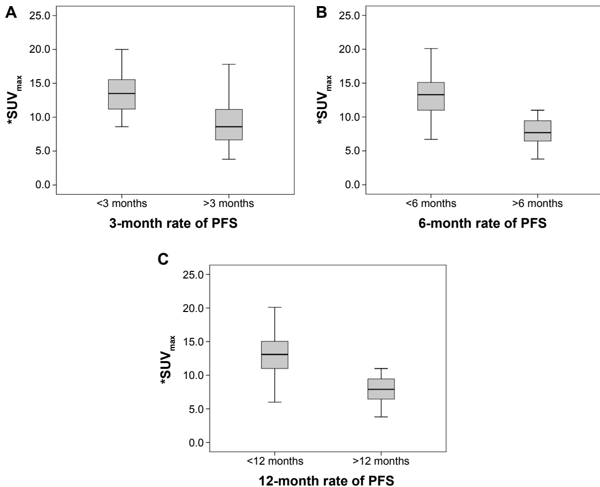
Figure 1 The (A) 3, (B) 6, and (C) 12-month rates of progression-free survival according to SUV max values. Note: *SUV max = decay corrected selected region activity (mCi/mL/injected dose [mCi]/body weight [kg]). Abbreviations: SUV max , maximum standardized uptake value; PFS, progression-free survival.
