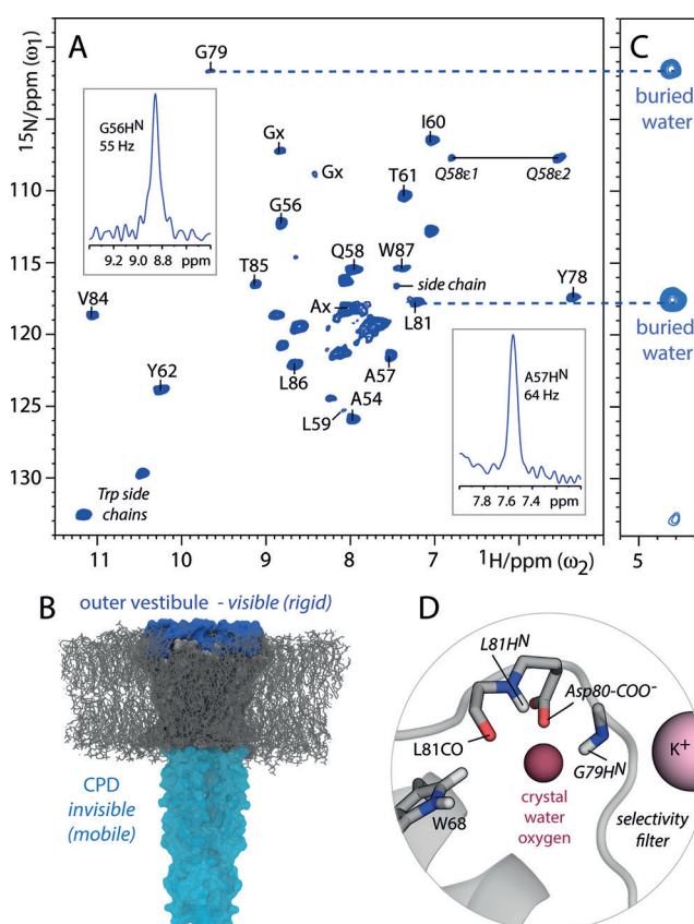
Figure 3. ^1\text{H} -detected studies with FD KcsA (closed-conductive).
