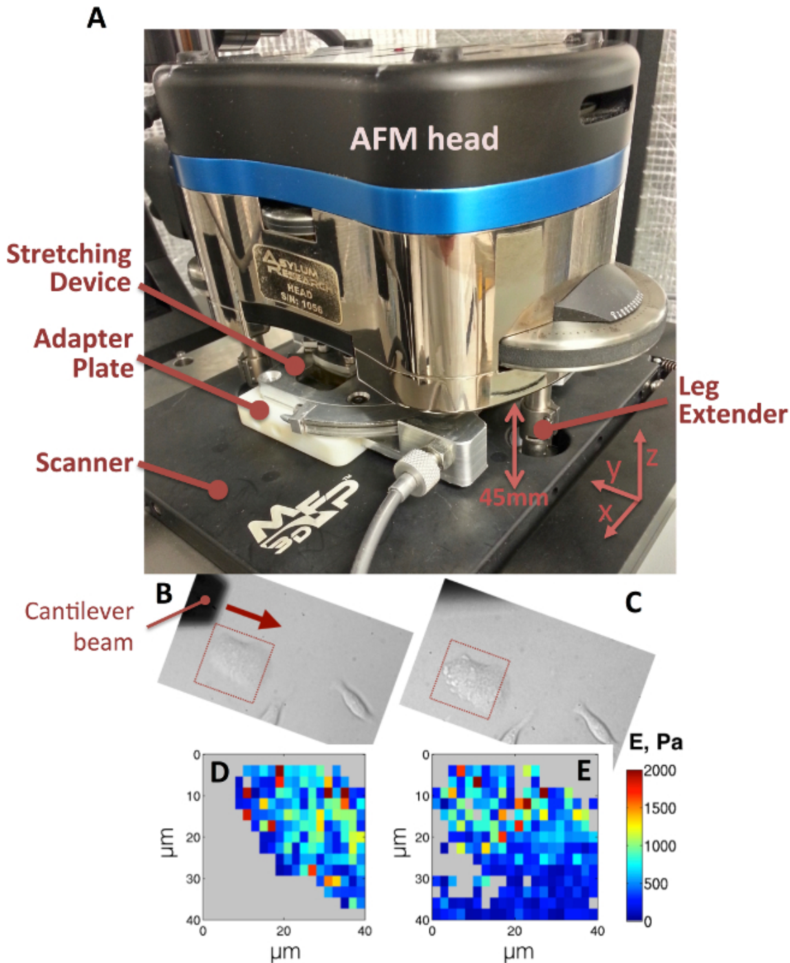
Figure 6. (A) Mechanical device shown in the AFM for nano-indentation of cells with stretch. The scanner must be removed for the placement of objective extender. Three leg extenders are attached to all three legs of the AFM head to allow for device placement. An adapter plate is utilized to mount the stretcher on to the AFM scanner (black plate). The cantilever beam scans in the direction of the arrow shown in the before stretch phase contrast image an MLE12 cell (B). The red squares in the before (B) and after (C) stretch images depict the area that was captured during nano-indentation (40X objective). The elastic modulus maps, before (D) and after (E) stretch, are obtained with previously published analysis techniques 13 . Please click here to view a larger version of this figure.
