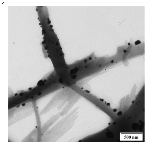
Fig. 11 TEM image of the Ag-loaded electrospun nanofibers. Ag NPs can be observed onto the ENFs surface. Reprinted with permission from [88]. Copyright (2012) Wiley Periodicals Inc
