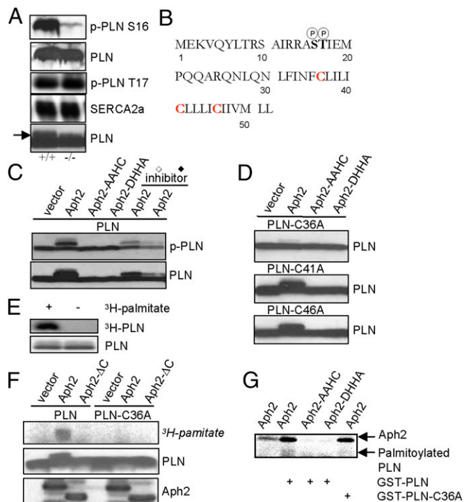
Fig. 3. Aph2 is a PAT for PLN. (A) Phosphorylation of PLN at Ser16 in newborn pups was reduced (see Fig. S3 C for quantitation data). Arrow indicates the slow migration band of PLN. (B) The protein sequence of mouse PLN, with potential palmitoylation sites marked in red. (C) Coexpression of Aph2 and PLN led to posttranslational modification of PLN, an activity depending upon the zf -DHHC domain. Aph2 and PLN were expressed in COS7 cells and analyzed by Western blot. This modification needed the DHHC motif and could be inhibited by 2BP (open diamond, 50 \mu M; filled diamond, 100 \mu M). (D) The modification occurred on Cys36 of PLN. The three cysteine residues were individually mutated to alanine. (E) Endogenous PLN of primary murine cardiomyocytes was modified by palmitoylation. Cardiomyocytes were cultured in the presence of 3 H-palmitic acid for 24 h, and endogenous PLN was immunoprecipitated, fractionated onto SDS/PAGE gels, and exposed to X-ray films. (F) In vivo labeling assay with 3 H-palmitic acid showed that Aph2 could modify PLN by palmitoylation, in a DHHC domain-dependent manner. (G) In vitro palmitoylation assay showed that Aph2 could directly palmitoylate PLN at Cys36 in a DHHA motif-dependent manner.
