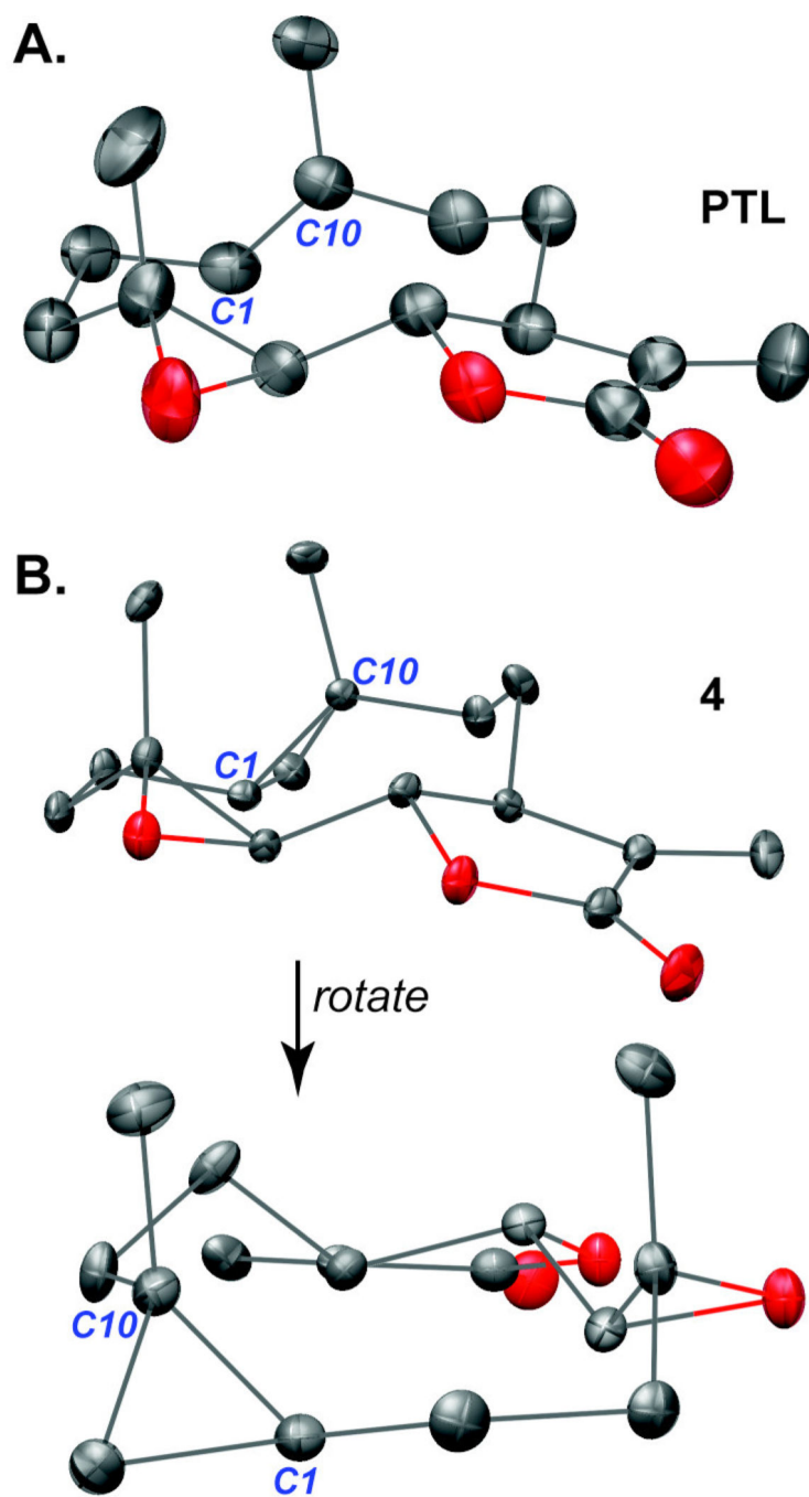
Figure 2. X-ray crystal structures. (A) PTL 18 and (B) cyclopropane 4 adopt similar conformations in the solid-state. Root-mean-square deviation between the two structures is 0.167 Å.
