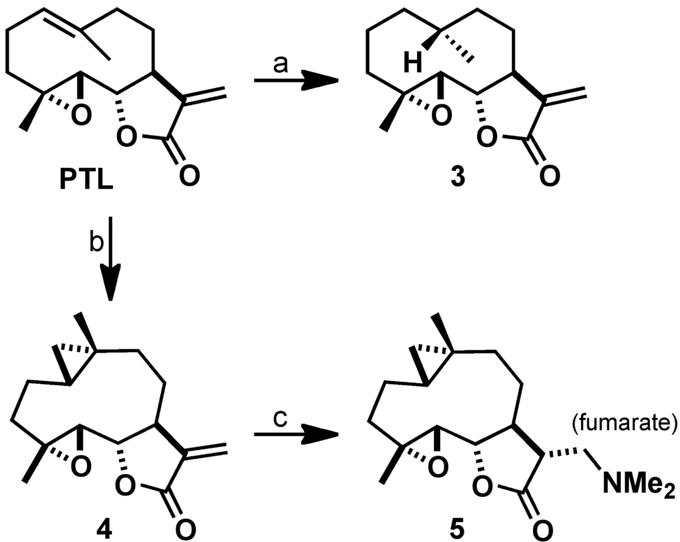
Scheme 1.
