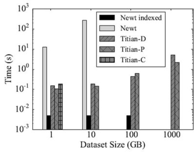
(a) L2 tracing time
