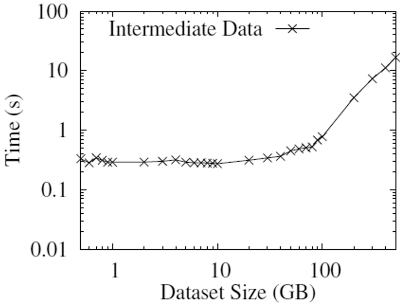
Figure 18. Data retrieval performance
