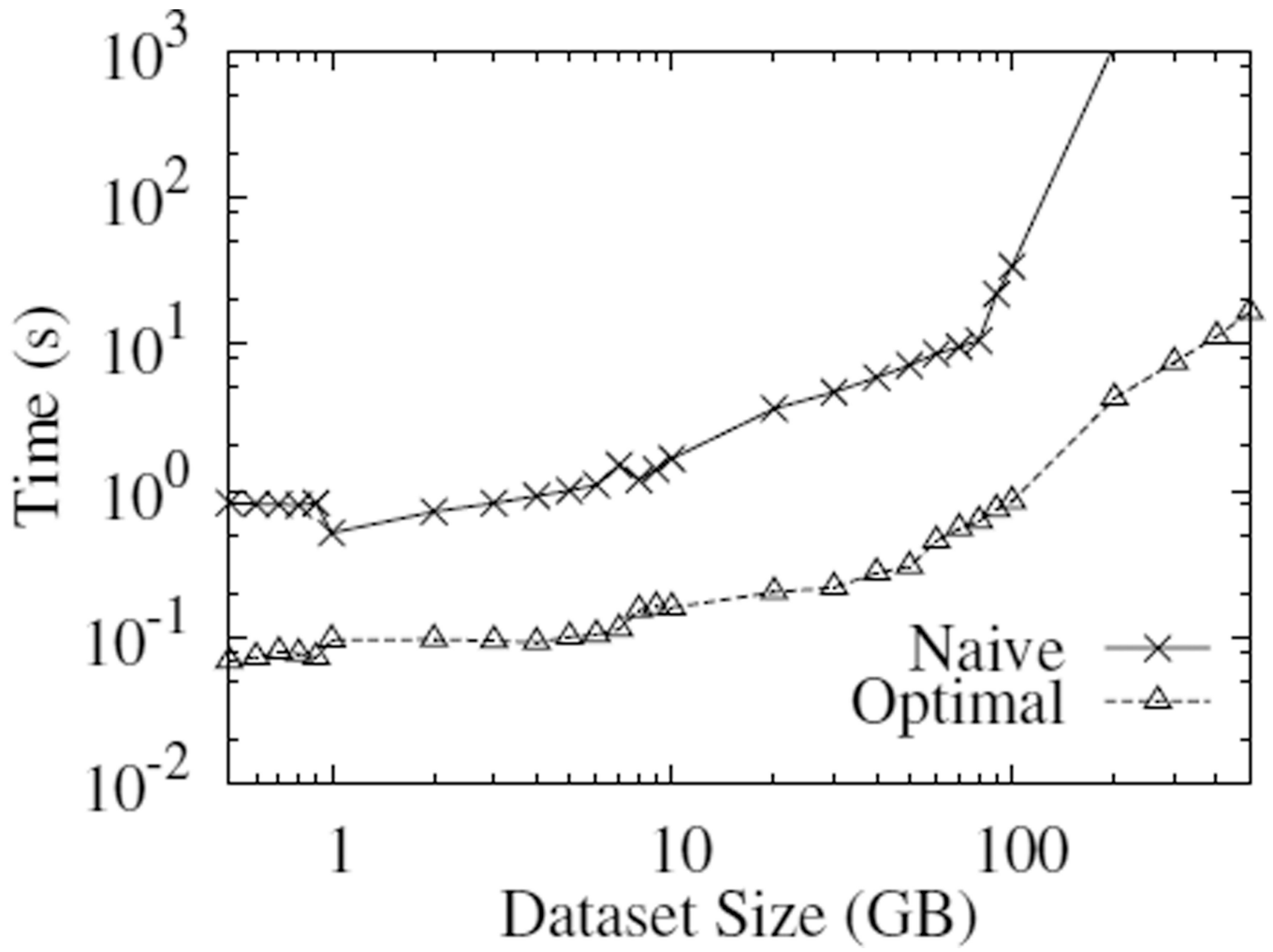
Figure 15. naïve vs optimal plan
