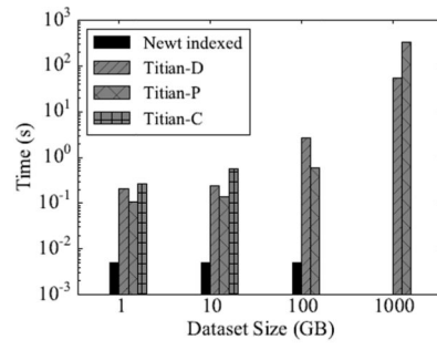
(b) L6 tracing time
