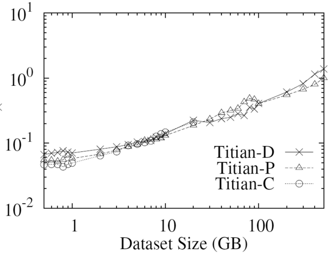
(b) Grep Titian versions
