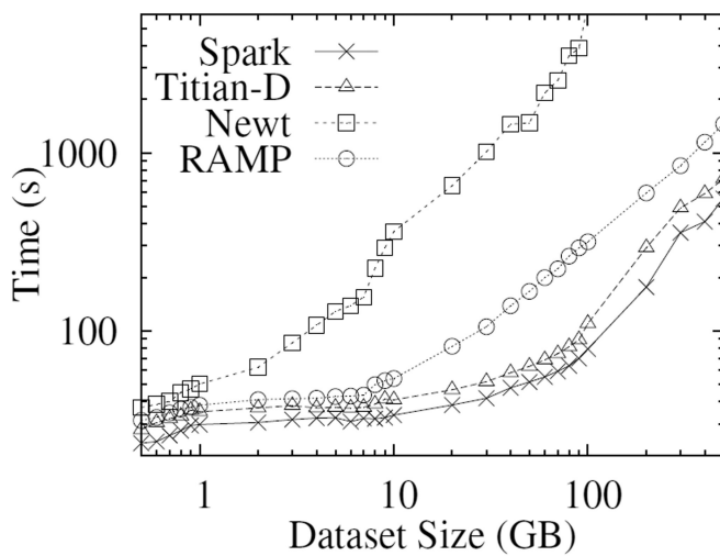
(c) WordCount distributed
