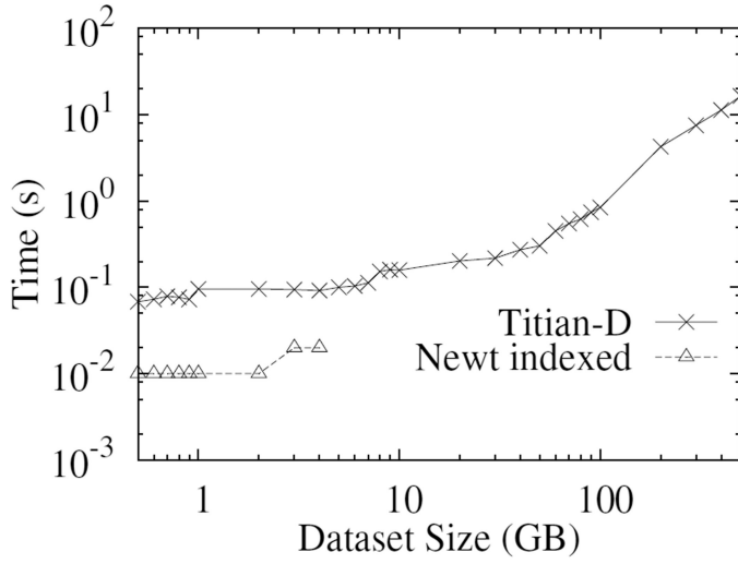
(c) WordCount distributed
