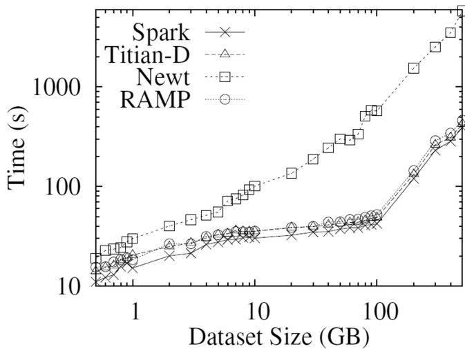
(a) Grep distributed
