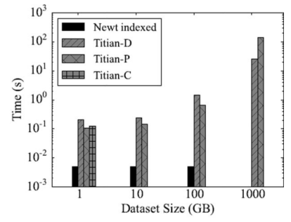
(c) L7 tracing time
