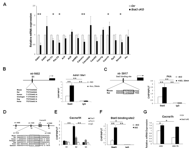
Figure 6. \beta AR signaling components as direct targets of STAT3. A , Quantitative RT-PCR analyses of \beta AR signaling components and calcium handling genes from hearts of 2-month old control and Stat3cKO mice (N = 3/each group). Ribosomal protein L7 mRNA was used for normalization. B , Positive regulation of Adrb1 by STAT3. Chromatin immunoprecipitation (ChIP) analysis of the STAT3 binding site in the promoter region of Adrb1 at nt-1602 relative to the transcription start site (TSS). C , Positive regulation of Prkaca by STAT3. ChIP analysis of the STAT3 binding site in the promoter region of Prkaca at nt-5917 relative to its TSS. D , Schematic diagram of putative STAT3 binding sites at the promoter region of Cacna1h . E–F , ChIP assay in combination with quantitative PCR demonstrates the active STAT3 binding site and its response to ISO stimulation. G , Cacna1h expression in 2-month old control and Stat3cKO hearts with or without dobutamine treatment (1 \mu g/g bodyweight), *P<0.05, **P<0.01.
