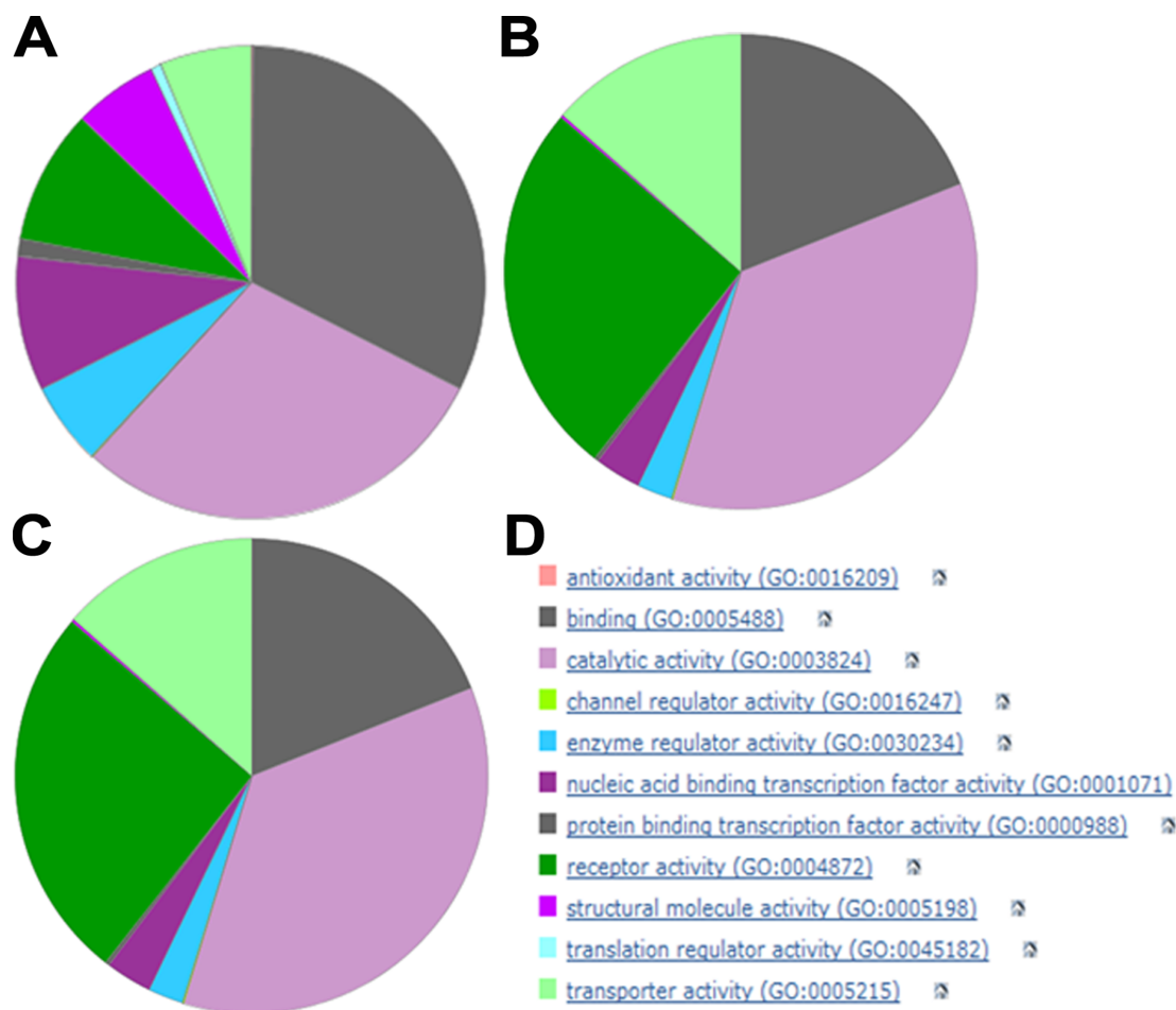
Figure 2. High level Gene Ontology (GO) functional categories for three sets of human proteins. Set A was generated from the total proteome of 20,204. Set B represents the 1,228 targets with quantitative ligand binding data in GtoPdb. Set C represents the 554 targets where at least one approved drug is included in the ligand binding data. Panel D provides the colour key to the top-level GO categories. The charts were generated by loading Swiss-Prot IDs from the protein sets into the PANTHER Gene List Analysis Tool (55).
