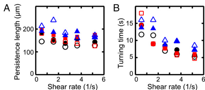
Fig. 2. Characteristics of the turning process for the cell trajectories in Fig. 1, using the same color coding for viscosities, with filled (unfilled) symbols indicating right-turning (left-turning) trajectories. (A) The persistence length \Lambda , defined as the maximum of the x component of each mean trajectory in Fig. 1A, shows weak variation with shear rate \dot{\gamma} . (B) The mean turning time T , defined as the time after which the x component of a mean trajectory reaches its maximum, is approximately inversely proportional to the shear rate, T \propto 1/\dot{\gamma} .
