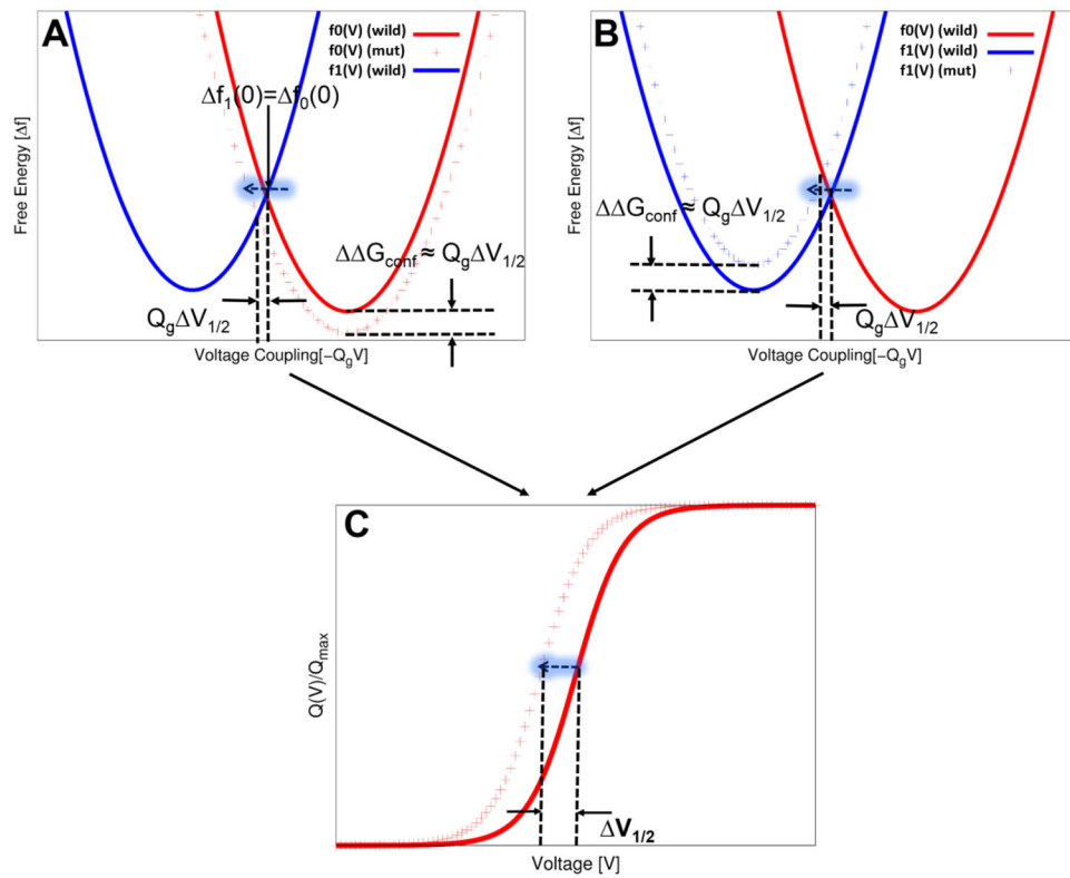
Figure 6. Schematic illustrations of the quantitative correlation between free energy landscapes (parabolas) and a Q-V curve. (A) The stabilization of an open activated state, for example, upon mutations and drug binding, leads to a left shift (toward hyperpolarization) in the Q-V curve (C). (B) The destabilization of a closed resting state also results in the same shift in the Q-V curve. The shift in the Q-V curve in terms of V_{1/2} is correlated with the stabilization or destabilization of the conformational states, with a quantitative relation of the form, Q_g V_{1/2} \approx \Delta G_{\text{conf}} (see Eq. 20).
