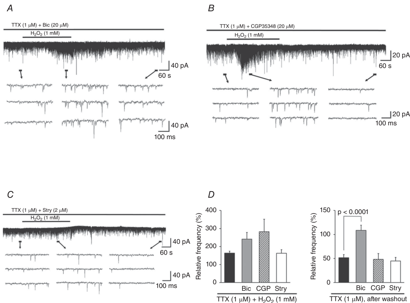
Figure 5. Effects of GABA and glycine receptor antagonists on \text{H}_2\text{O}_2 -induced changes in mEPSC frequency
