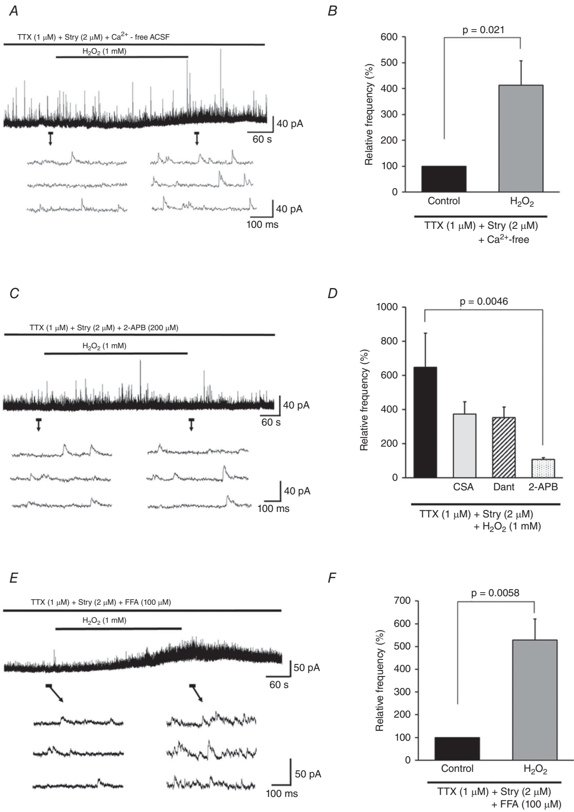
Figure 7. H 2 O 2 -induced increase in GABAergic mIPSC frequency is due to intracellular Ca 2+ release via IP 3 R
