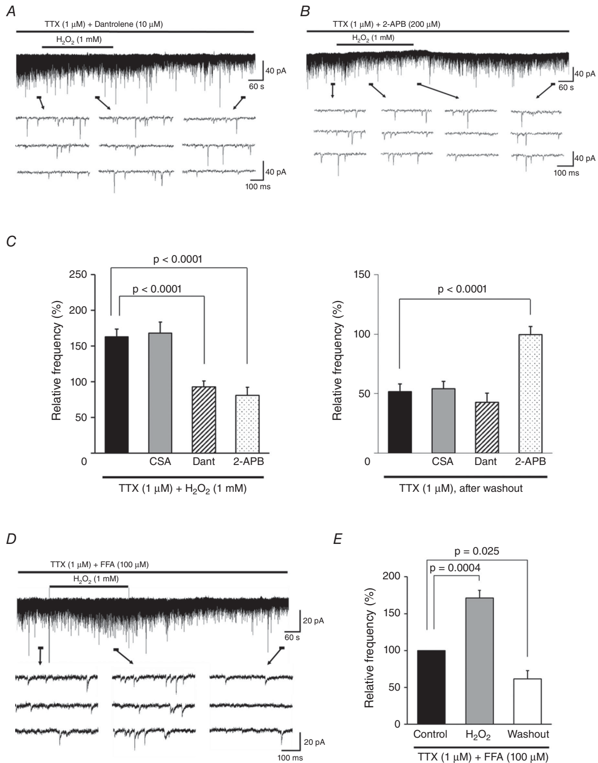
Figure 4. H 2 O 2 -induced increases in mEPSC frequency are due to intracellular Ca 2+ release via RyR and IP3R
