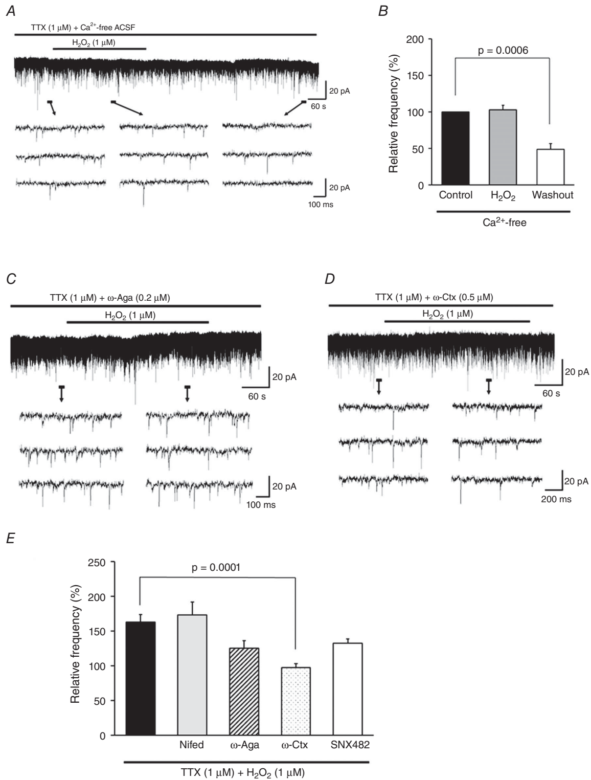
Figure 3. H 2 O 2 induces an increase in mEPSC frequency by modulating Ca 2+ influx via N-type VGCCs
