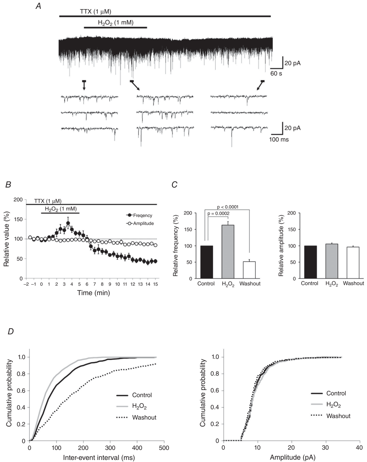
Figure 1. H 2 O 2 induces an increase followed by depression in mEPSC frequency without affecting amplitude
