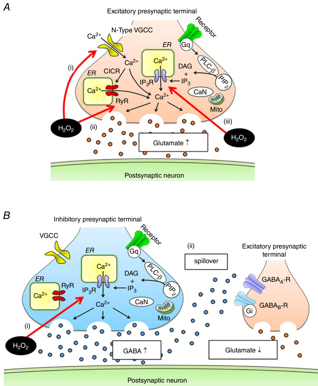
Figure 8. Model of H_2O_2 -induced modulation of presynaptic activity in spinal VH neurons
