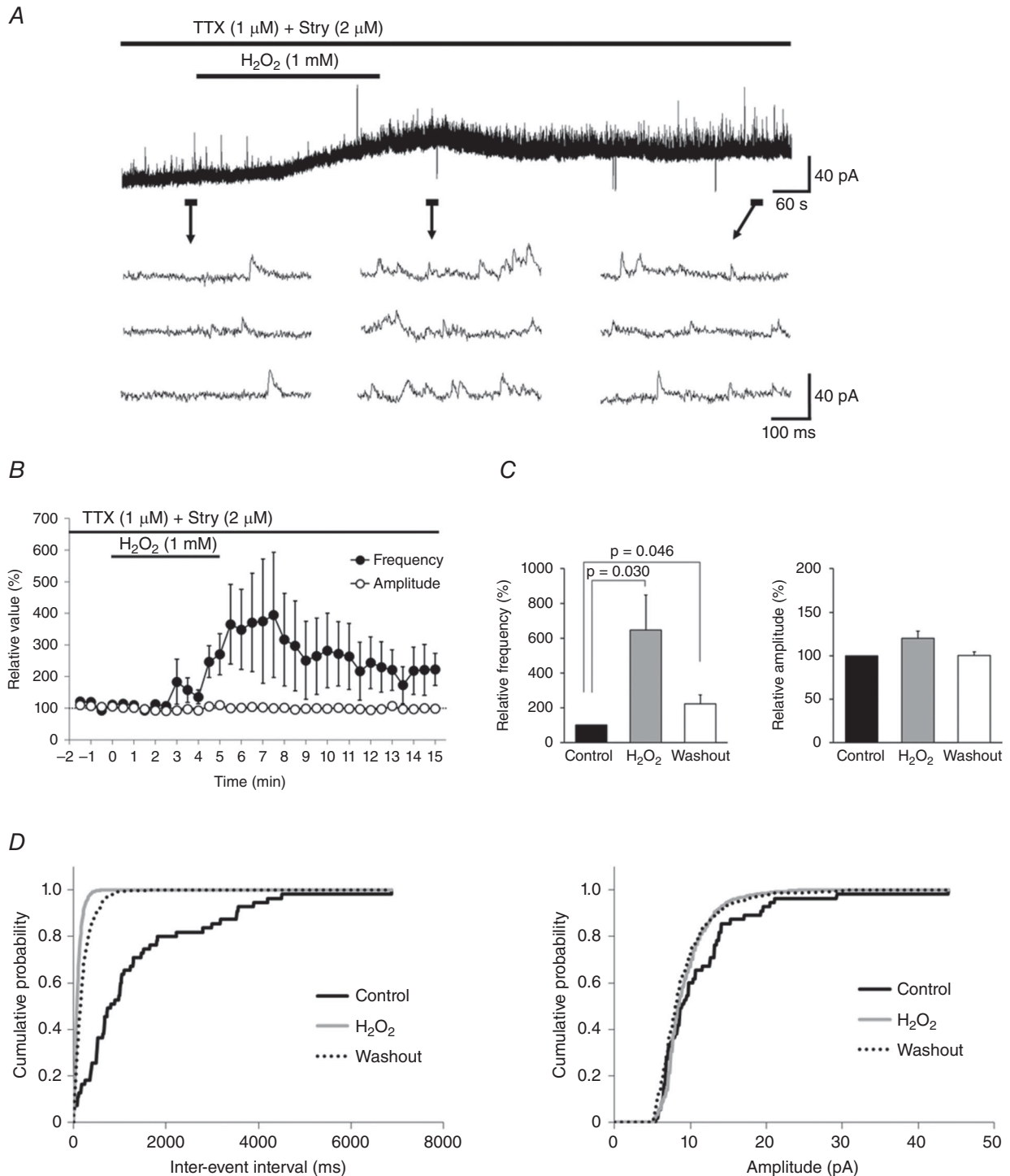
Figure 6. H 2 O 2 increases the frequency of GABAergic mIPSCs
