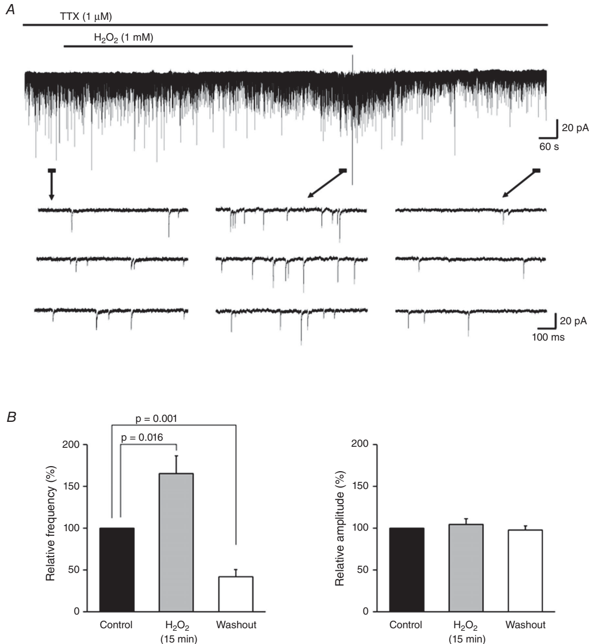
Figure 2. Prolonged application of H 2 O 2 results in an increase followed by depression in mEPSC frequency
