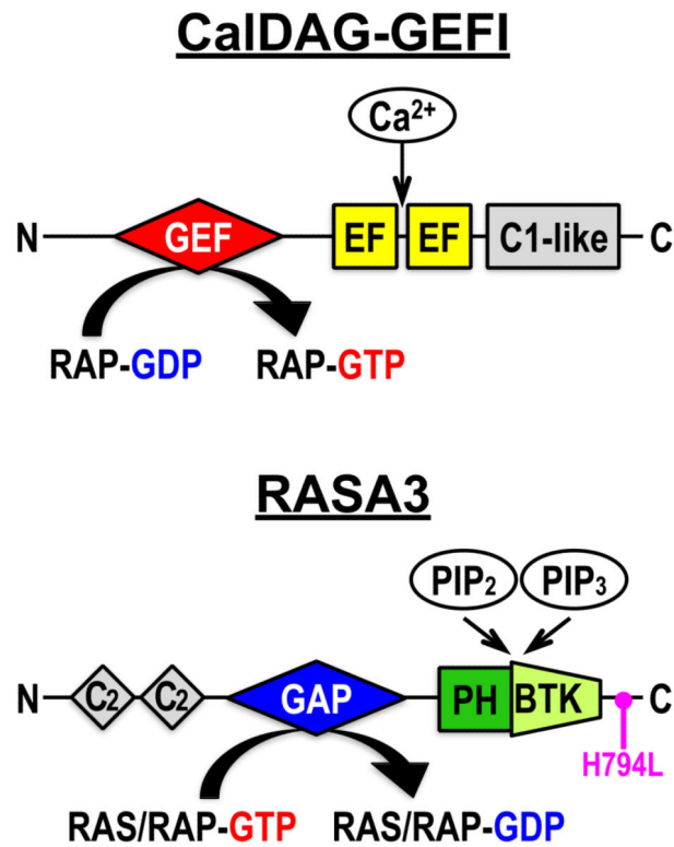
Fig.2. Domain structure of the RAP1 regulators, CaIDAG-GEFI and RASA3
