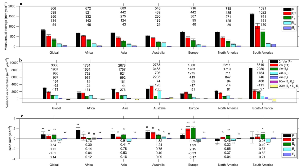
Figure 4. Mean global land surface and continental averages (1981–2012) of various statistics for P, ET, E t , E s , and E i . (a) Mean annual values (mm year -1 ). (b) Variance or covariance of annual values (mm 2 year -2 ). (c) Trend (mm year -2 ). Error bars are s.d. obtained from PML simulations 1 and 2. The symbol ** indicates significance level 1-\alpha = 99\% ( p < 0.01 ); the symbol * indicates significance level 1-\alpha = 95\% ( p < 0.05 ); the symbol 'n' is not significant ( p > 0.05 ). In each figure sub-part for each geographic area the numbers presented are ordered equivalently to the sub-part legend. Note that scaling is applied to the Var (P) on part (b).
