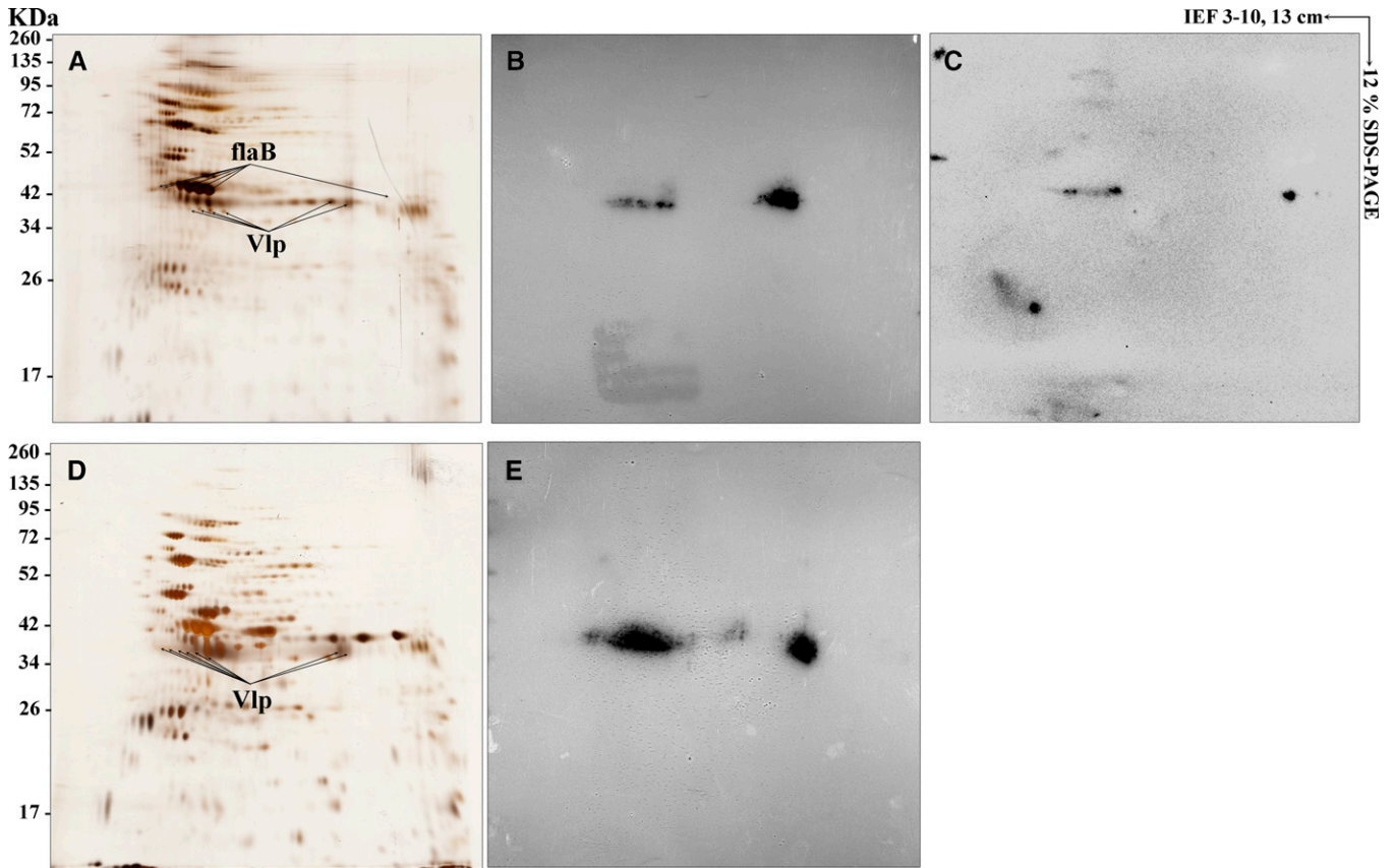
FIGURE 3. Immunoreactive proteins with mouse monoclonal antibodies (MAbs) P6D9 and P3A10. Borrelia crocidurae and Borrelia duttonii proteins were resolved in the first dimension over an isoelectric point gradient of 3–10 followed by 12% linear sodium dodecyl sulfate polyacrylamide gel electrophoresis for the second dimension. Proteins were then detected by silver staining (A and D for B. crocidurae and B. duttonii , respectively) or transferred to a nitrocellulose membrane and probed with purified mouse MAbs P6D9 (B and E) and P3A10 (C) at 1:1,000 dilution. Standard molecular weight markers are indicated on the left in kilodaltons (kDa). Identified immunoreactive proteins, achieved by matrix-assisted laser desorption/ionization time-of-flight analysis, are indicated by protein name.
