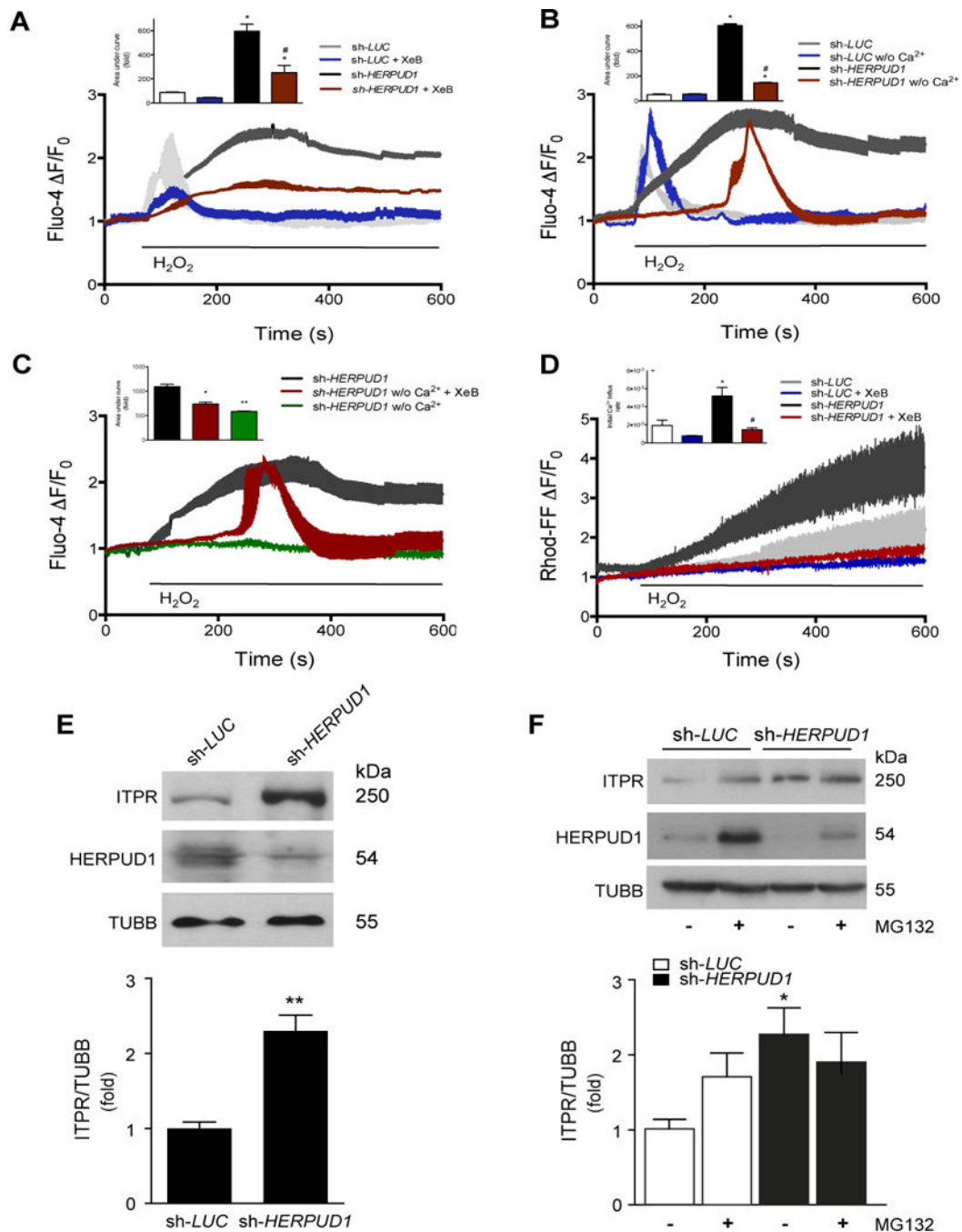
Fig. 3. HERPUD1 regulates intracellular and mitochondrial Ca 2+ by controlling ITPR protein levels. (A) sh- Luc (control) or sh- HERPUD1 HeLa cells were pretreated or not with xestospongin B (XeB, 100 \mu M, IP3R antagonist), preloaded with Fluo-4AM (5.4 \mu M, cytosolic Ca 2+ probe) for 30 min, treated with H 2 O 2 and then visualized under a confocal microscope. Insert: Quantitation of the area under the curve of the kinetics shown in the Figure. (B) sh- Luc (control) or sh- HERPUD1 HeLa cells were preloaded with Fluo-4AM (5.4 \mu M) and incubated in Ca 2+ -containing (w/Ca 2+ ) or Ca 2+ -free (w/o Ca 2+ ) resting media. (C) sh- HERPUD1 HeLa cells were preloaded with Fluo-4AM (5.4 \mu M) and incubated in Ca 2+ -free resting media. (D) sh- HERPUD1 HeLa cells were preloaded with Rhod-FF (5.4 \mu M) and incubated in Ca 2+ -containing resting media. (E) Western blot analysis of ITPR, HERPUD1, and TUBB protein levels in sh- Luc and sh- HERPUD1 HeLa cells. (F) Western blot analysis of ITPR and TUBB protein levels in sh- Luc and sh- HERPUD1 HeLa cells treated with MG132.
