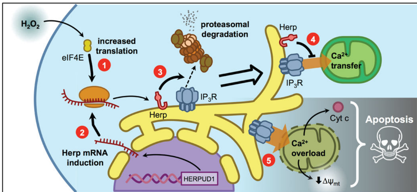
Fig. 6. Model of cell protection mediated by HERPUD1 against H_2O_2 -induced apoptosis. (1) H_2O_2 induces a fast HERPUD1 (Herp) protein-level increase by transduction of preformed mRNA through an eIF4E-dependent mechanism and (2) a slow increase mediated by a transcriptional mechanism. (3) HERPUD1 induces inositol 1,4,5-trisphosphate receptor (IP 3 R) degradation by proteasome. (4) HERPUD1 reduces Ca^{2+} release from the endoplasmic reticulum, (5) reducing Ca^{2+} overload in the mitochondria, impeding mitochondrial transition pore opening and decreasing apoptosis.
