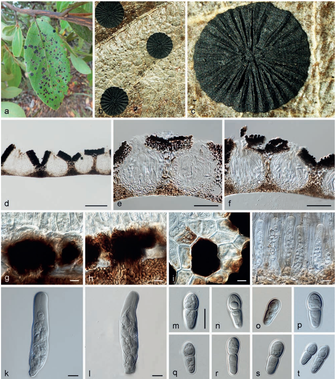
Fig. 2 Parmularia styracis VIC 42447. a. Living leaves of Styrox ferrugineus with epiphyllous colonies; b, c. detail of the mature colony, opening by radiating fissures; d. vertical section showing entirely superficial ascoma with fertile locules; e, f. detail of the fertile locules; g, h. hyphal columns which connect the colony with the host tissue; i. horizontal section showing the detail of a tuft of internal mycelium that ruptures the cuticle and produce the initial stages of the ascostromata; j. detail of the fertile locule with fully developed asci and pseudoparaphyses; k, l. asci; m–t. ascospores. — Scale bars: d = 100 \mu m; e, f = 50 \mu m; g–m = 10 \mu m.
