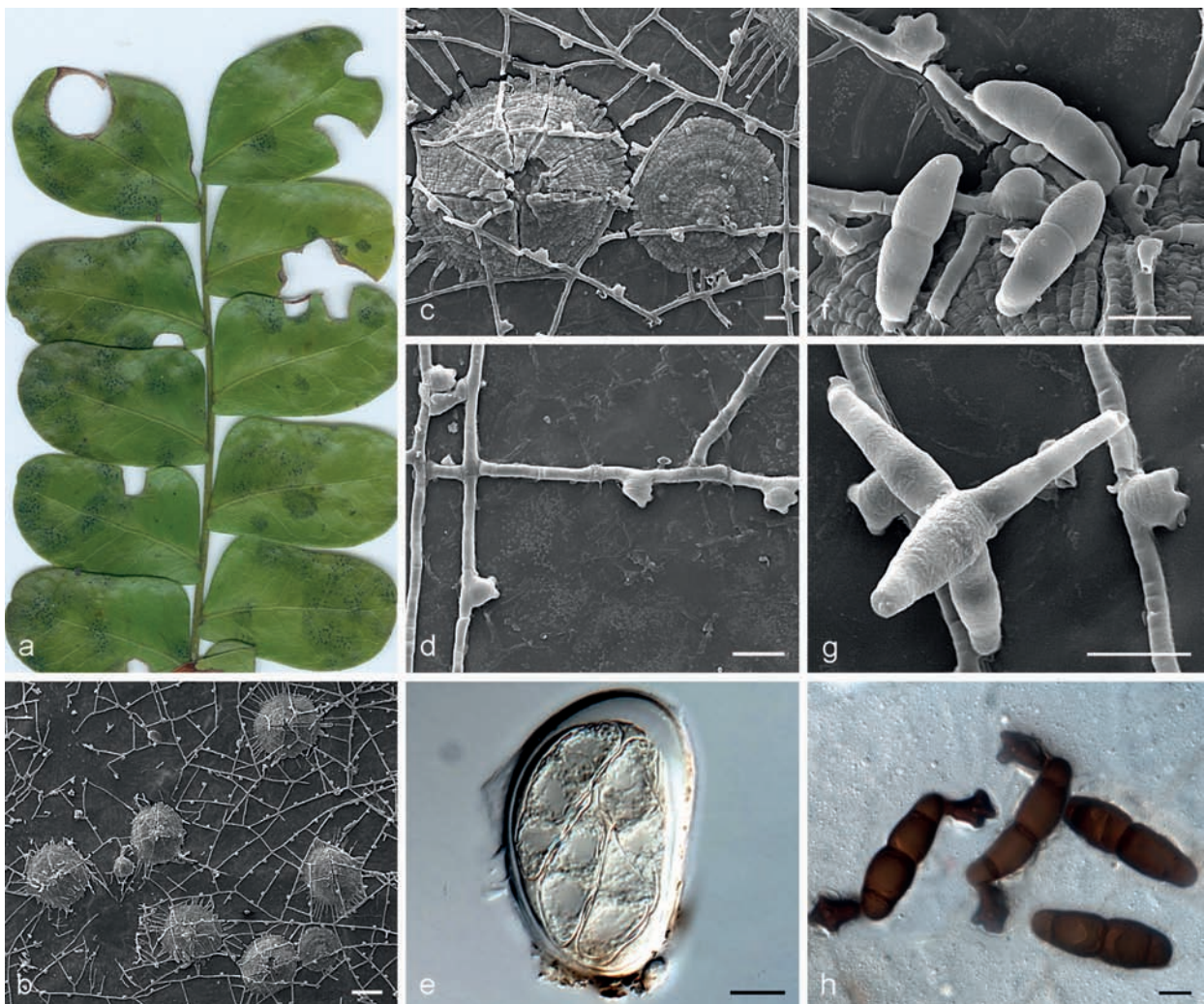
Fig. 5 Batistinula gallsiae VIC 42514. a. Living leaves of Caesalpinia echinata with epiphyllous colonies; b–d, f, g. SEM images: b. colony with open thyriothecia and external mycelium; c. thyriothecium opened by a central star-shaped fissure; d. appressoria straight, lobate, cylindrical, unicellular; e. asci ovoid, showing immature ascospores; f. ascospores oblong, with ends broadly rounded, constricted at the septum; g. conidia of Tripodsporium (asexual morph) and erect conidiophore; h. ascospores with lobate appressoria. — Scale bars: b = 100 µm; c, d, f, g = 20 µm; e, h = 10 µm.
