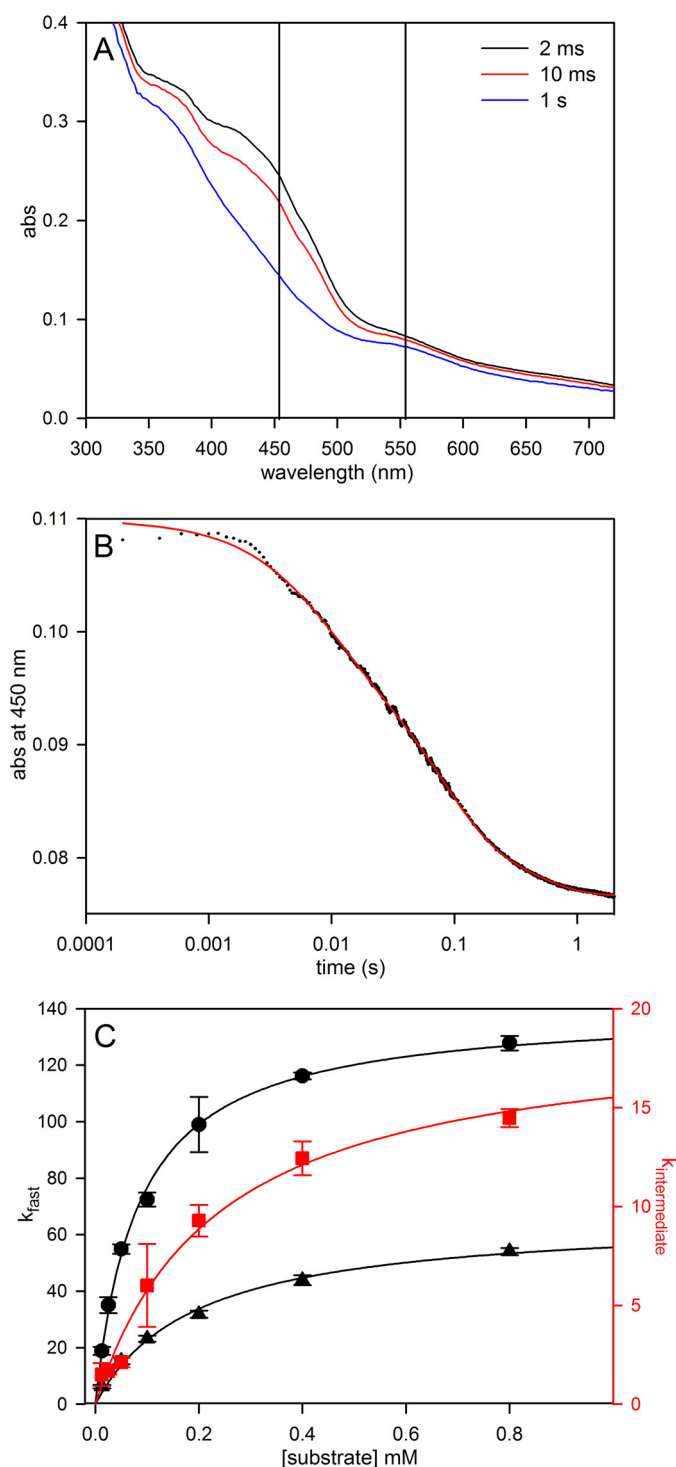
FIGURE 3. Pre-steady-state kinetics for the reduction of FdsABG with formate or [\text{2H}] formate. A , rapid scanning stopped flow traces for the reaction of 6 \mu\text{M} of FdsABG with 5 \text{ mM} formate performed at 10^\circ\text{C} in 75 \text{ mM} \text{K-PO}_4 , pH 7.7. B , a representative kinetic trace of the reaction of FdsABG with 0.8 \text{ mM} sodium formate monitored at 450 \text{ nm} . The trace is best represented by three phases with k_{\text{obs}} = 124, 14, \text{ and } 2.5 \text{ s}^{-1} , with \Delta A = 0.011, 0.017, 0.006 , respectively. C , plots of k_{\text{fast}} (black circles) and k_{\text{intermediate}} (red squares) versus formate concentrations or k_{\text{fast}} (black triangles) versus [\text{2H}] formate concentrations. All reactions were performed at 10^\circ\text{C} in 75 \text{ mM} \text{K-PO}_4 , pH 7.7, with 2.5 \mu\text{M} FdsABG. Hyperbolic fits (solid lines) yielded k_{\text{fast}} = 140 \text{ s}^{-1} , K_d^{\text{formate}} = 82 \mu\text{M} , k_{\text{intermediate}} = 19 \text{ s}^{-1} , and K_d^{\text{formate}} = 230 \mu\text{M} for reaction with formate and k_{\text{fast}} = 66 \text{ s}^{-1} , and K_d^{[\text{2H}] \text{formate}} = 193 \mu\text{M} for reaction with [\text{2H}] formate.
