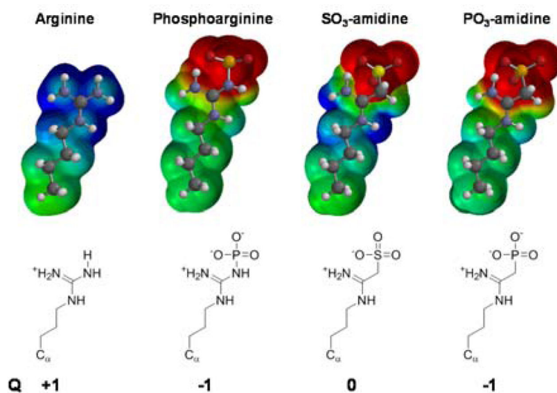
Figure 1. Structural representation of the electrostatic map of the side chain of arginine, phosphoarginine and its stable analogs SO 3 -amidine as well as PO 3 -amidine. The formal net charge of the individual compounds is denoted by Q.
