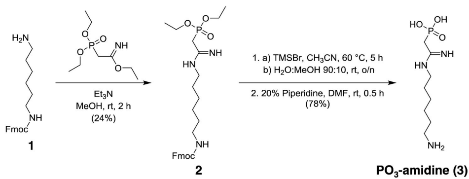
Scheme 1. Synthesis of PO 3 -amidine (3) (2-((6-aminohexyl)amino)-2-iminoethyl)phosphonic acid.
