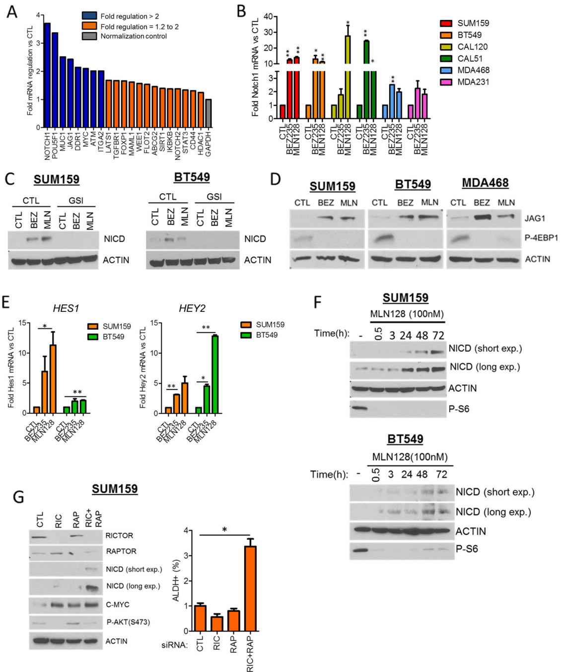
Figure 2. TORC1/2 inhibition increases Notch1 expression and activity in TNBC cell lines (A) SUM159 cells were treated with control or 100 nM MLN128 for 48 h. RNA was extracted and used in the Cancer Stem Cell-specific PCR Array. Fold regulation of gene expression changes in MLN128-treated cells vs CTL was determined using the SA Biosciences PCR Array Software. (B) SUM159, BT549, CAL120, CAL51, MDA468 and MDA231 cells were treated with 250 nM BEZ235 or 100 nM MLN128 for 72 h. Q-PCR analysis was performed for NOTCH1 (*P<0.05; **P<0.005).
