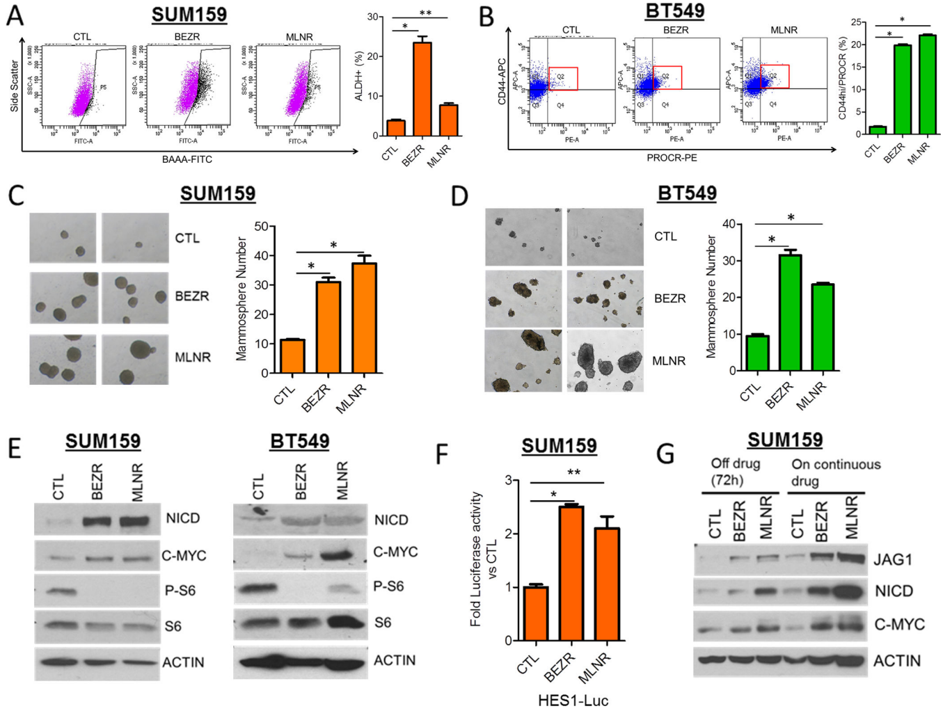
Figure 3. Persistent TORC1/2 inhibition drives Notch1 signaling and a CSC-like phenotype (A) SUM159 and (B) BT549 cells were treated with progressively higher concentrations (5–300 nM) of BEZ235 (BEZR) and MLN128 (MLNR) over a period of 8 weeks. FACS analysis for the CSC markers were quantified (SUM159: *P=0.0002, **P=0.002; BT549: *P<0.03).
