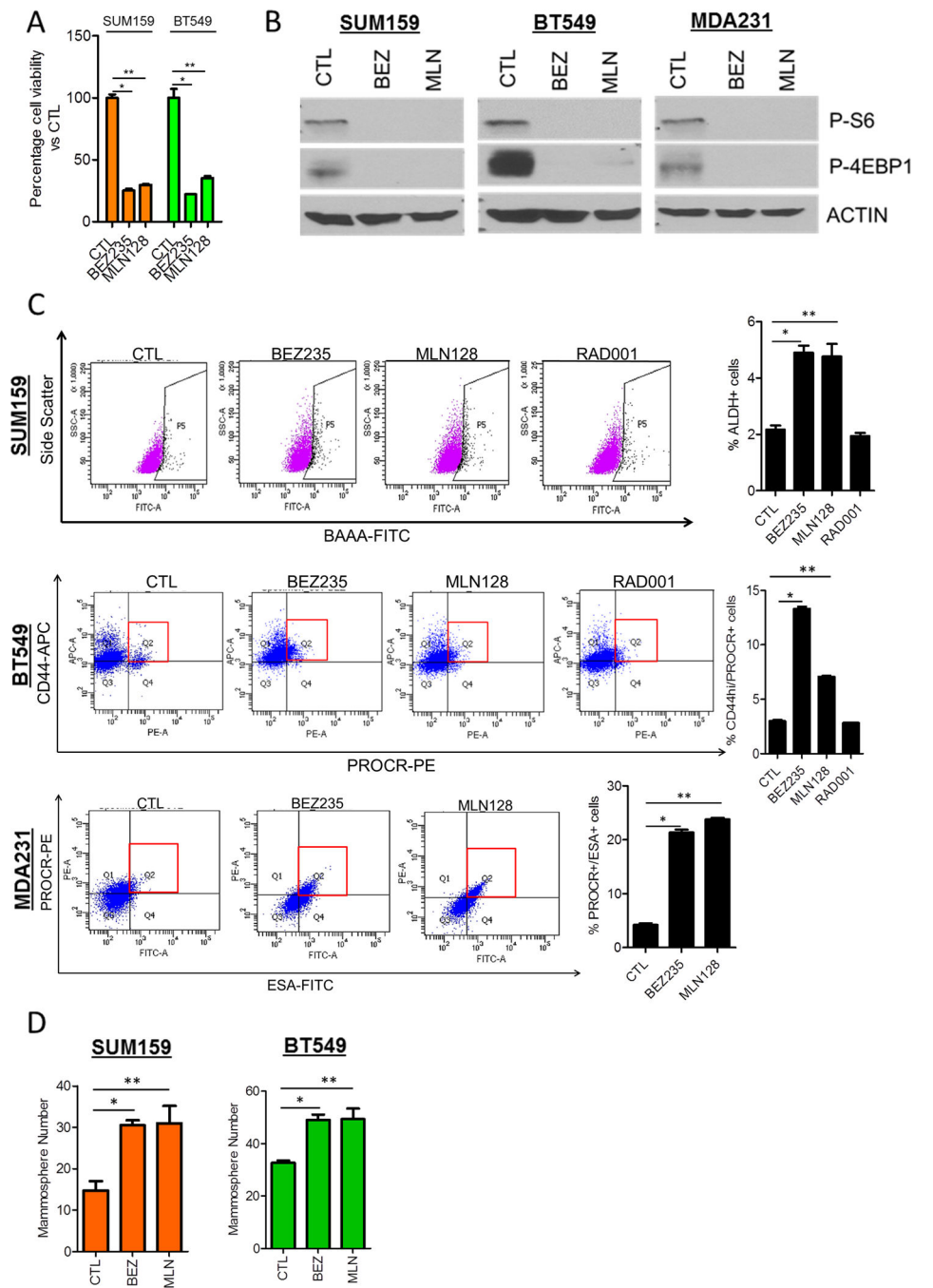
Figure 1. PI3K/mTOR and TORC1/2 inhibitors enrich for a CSC population in TNBC cell lines (A) SUM159 and BT549 cells were treated with 250 nM BEZ235 or 100 nM MLN128 for 72h. Cell viability was determined by the Alamar Blue viability assay (*P<0.009, **P<0.02). (B) SUM159, BT549 and MDA231 cells treated for 72 h were analyzed for phosphorylated S6 and 4EBP1 by immunoblot analysis. (C) SUM159, BT549 and MDA231 cells were treated with 250 nM BEZ235, 100 nM MLN128 or 100 nM RAD001 for 72 h. FACS analysis for CSC markers (SUM159-ALDH+,
