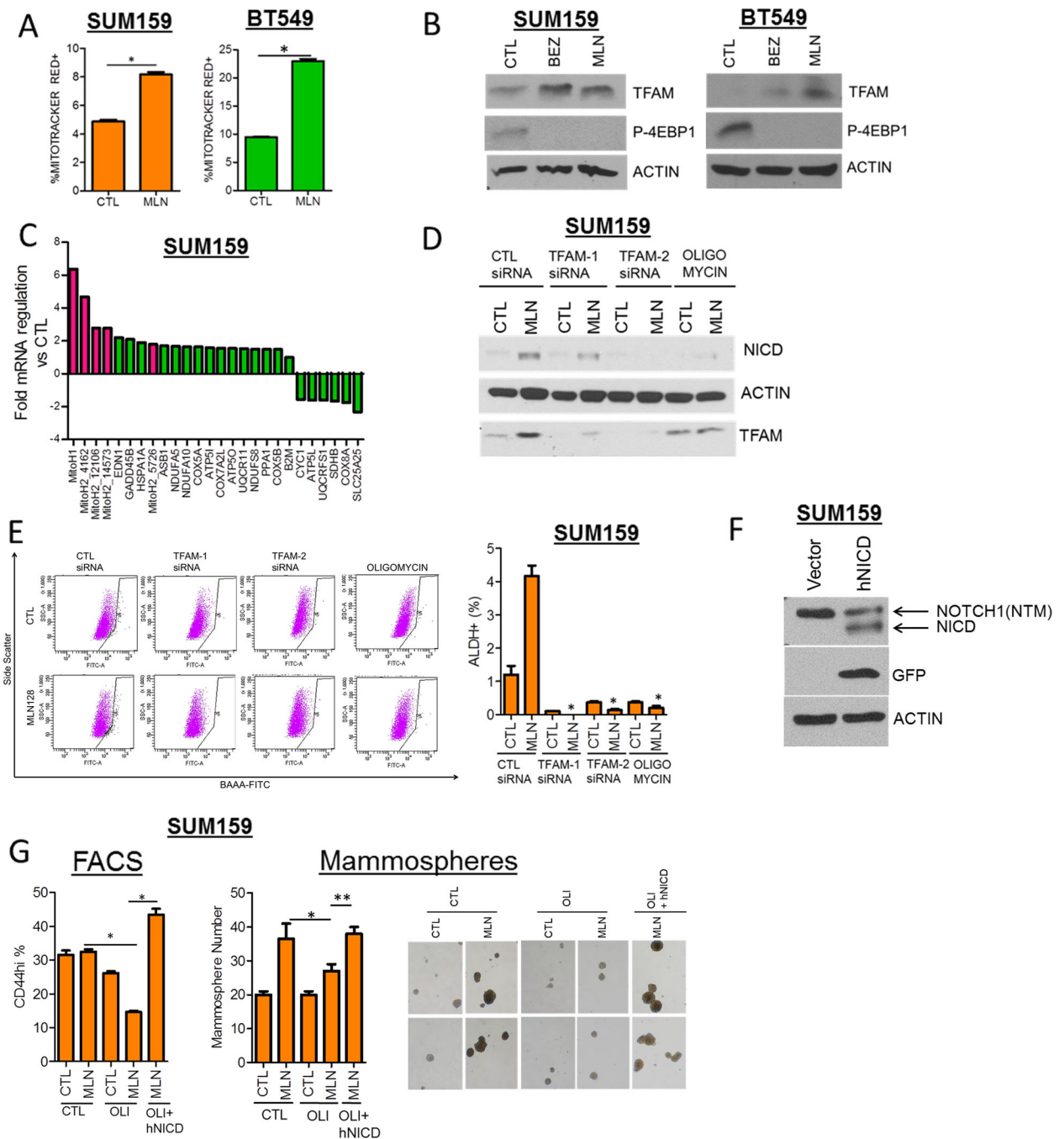
Figure 5. Induction of NICD and CSCs following TORC1/2 inhibition is dependent on mitochondrial metabolism (A) SUM159 and BT549 cells were treated with control or 100 nM MLN128 for 48 h. Cells were stained with a marker for mitochondrial membrane potential Mitotracker Red-CMXRos and analyzed by flow cytometry. Percentage of Mitotracker Red-positive cells was determined (*P<0.0008). (B) SUM159 and BT549 cells were treated with vehicle, 250 nM BEZ235 or 100 nM MLN128 for 72 h. Immunoblot analysis for TFAM, phospho-4EBP1, and Actin was performed.
