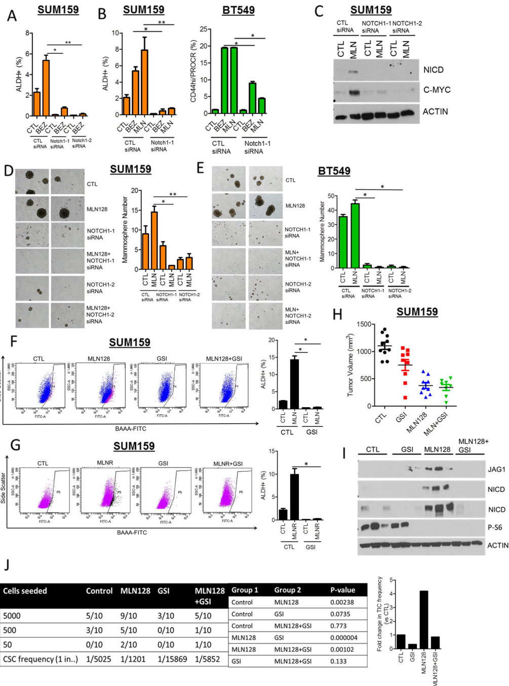
Figure 4. Notch1 downmodulation decreases the induction of CSCs upon inhibition of TORC1/2 (A) SUM159 cells were transfected with two different Notch1 siRNAs ± 250 nM BEZ235 for 72 h. FACS analysis for ALDH+ cells was performed (*P<0.03; **P<0.001). (B) SUM159 and BT549 cells were transfected with Notch1 siRNA ± 250 nM BEZ235 or 100 nM MLN128. After 72 h, FACS analysis for ALDH+ or CD44hi/PROCR+ expression was performed (*P< 0.03; **P<0.001). (C) SUM159 cells were transfected with 2 Notch1 siRNAs ± 100 nM MLN128. After 72 h, immunoblot analysis for NICD, C-MYC and Actin expression was performed.
