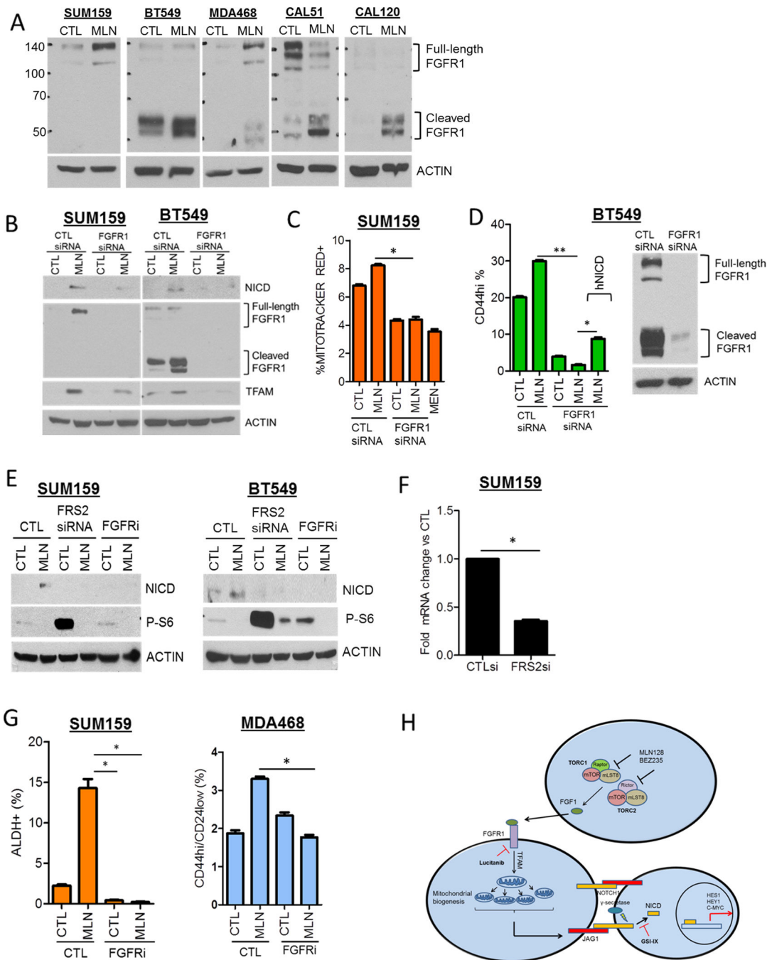
Figure 6. Induction of Notch1 and CSCs upon inhibition of TORC1/2 is FGFR-dependent (A) SUM159, BT549, MDA468, CAL51, and CAL120 cells were treated with 100 nM MLN128 for 72 h. Immunoblot analysis for FGFR1 and actin was performed. (B) SUM159 and BT549 cells were transfected with control or FGFR1 siRNA ± 100 nM MLN128 for 72 h. Immunoblot analysis for NICD, FGFR1, TFAM and Actin was performed.
