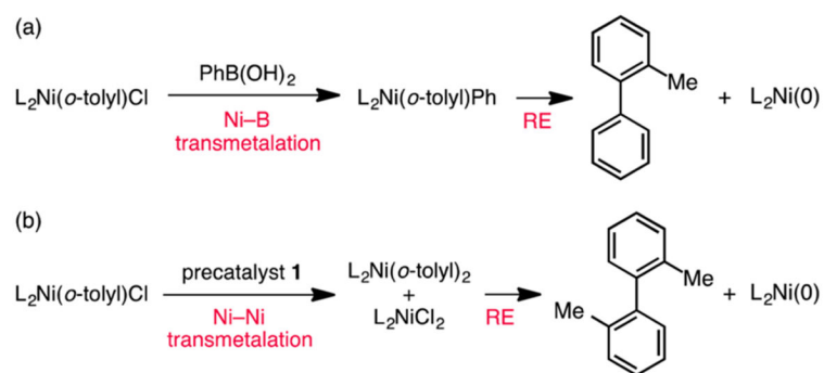
Scheme 2. Mechanisms for Precatalyst Activation
