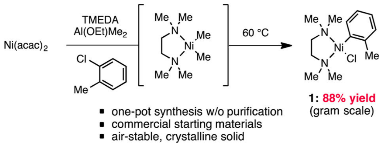
Scheme 1. Synthesis of Nickel Precatalyst 1
