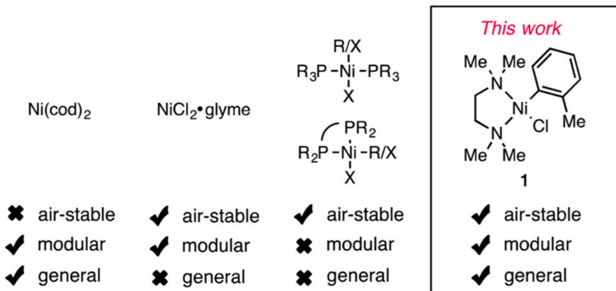
Figure 1. Prior art in nickel precatalysts.
