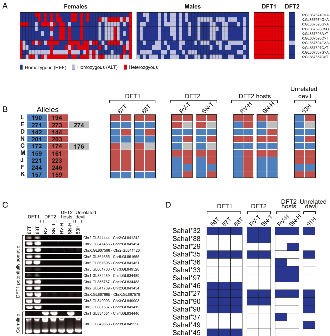
Fig. 4. DFT2 tumors are genetically distinct from DFT1 and from their hosts. (A) Genotyping of X-linked SNPs. Genotypes of 37 female and 37 male devils at 10 X-linked SNP loci that are heterozygous in DFT1. Both homozygous and hemizygous genotypes are referred to as homozygous. Each individual is represented by a column, and chromosome and scaffold for each locus is shown. Further information about individuals and exact SNP coordinates are available in Tables S3 and S4. (B) Microsatellite genotypes at nine polymorphic microsatellite loci (L, E, D, N, C, M, J, F, and K). The lengths of the two (L, D, N, M, J, F, and K) or three (E and C) alleles found at each locus and their color codes are shown on the left, and their genotypes in DFT1 tumors, DFT2 tumors, DFT2 hosts, and in 53H, a representative unrelated devil, are shown. All tumors are presented as diploid, although true copy number at these loci is not known. Further information about allele sizes is found in Table S2. (C) Structural variant genotyping. PCRs spanning breakpoint junctions were performed to assess the presence or absence of twelve possibly somatic structural variants and two polymorphic germ-line variants. We cannot confirm if structural variants found only in DFT1 are somatic or rare germ-line variants, thus these are labeled potentially somatic. Chromosomes and scaffolds involved in each rearrangement are indicated, and full breakpoint coordinates are available in Table S5. (D) MHC class I exon 2 haplotypes detected in DFT1 tumors, DFT2 tumors, DFT2 hosts, and in 91H, a representative unrelated devil. Exon 2 haplotype names are indicated on the left, and their presence or absence in the panel of samples are indicated with blue and white squares respectively. All 14 haplotypes are predicted to encode a unique amino acid sequence. Complete sequences for each haplotype are available in Tables S6 and S7.
