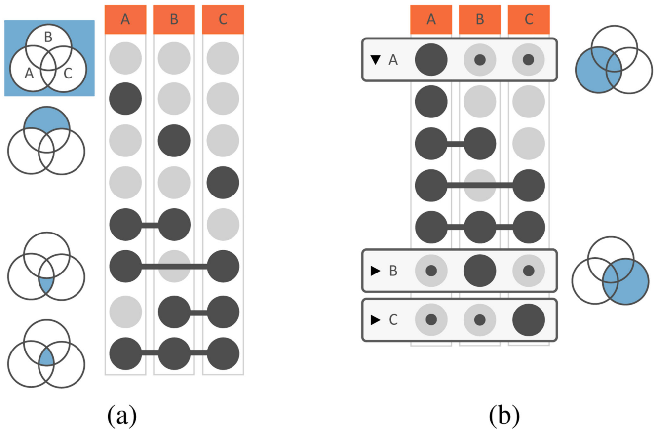
Fig. 6. The combination matrix encoding the relationships between sets, aggregates and exclusive intersections. (a) Each row corresponds to an exclusive intersection that contains the elements of the sets represented by the dark circles, but not of the others. The equivalent segment in a Venn diagram is shown on the left. (b) Aggregates group exclusive intersections meaningfully. The first aggregate shows its contained exclusive intersections, while the second and the third aggregates are collapsed.
