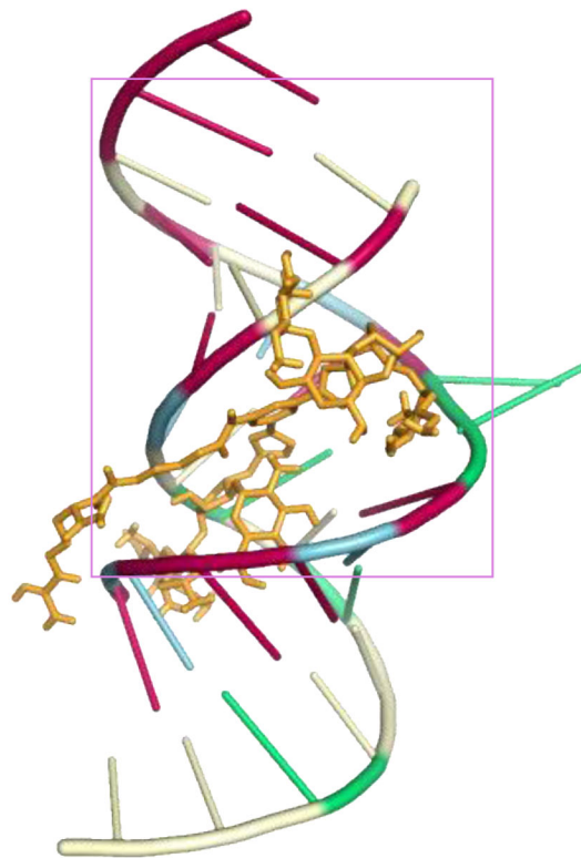
E. coli A-site with cpd 11
