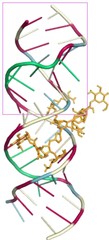
Human cytosolic A-site with cpd 11
