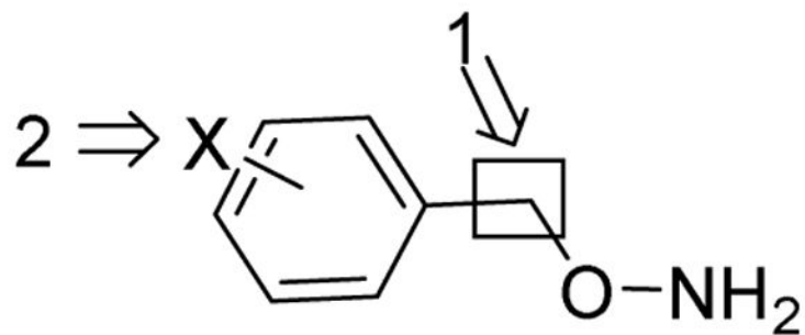
Figure 2. Two Modifications of O-Benzylhydroxylamine Lead Compound
