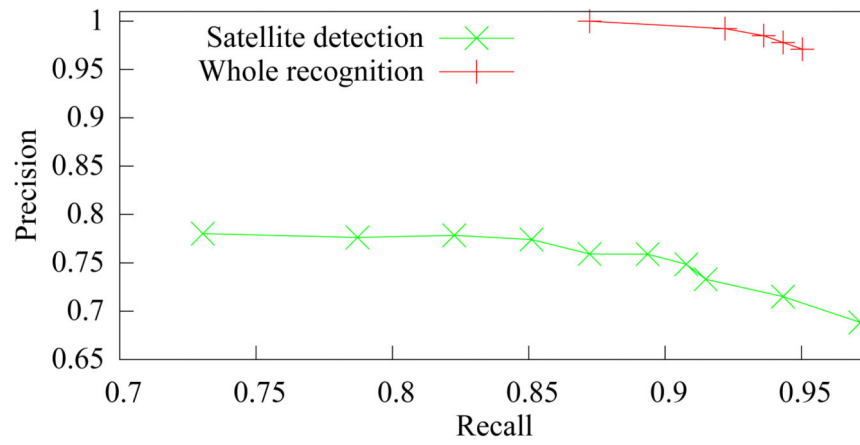
Figure 8. Pareto frontier of the detection procedure
