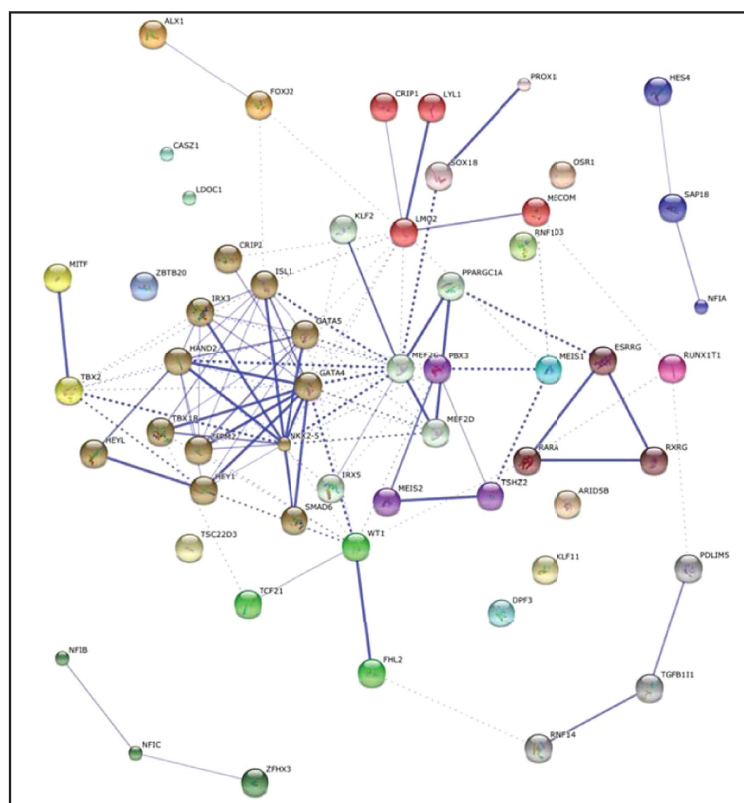
Figure 6. Enriched transcripts at day 10 and day 14 of differentiation in MESP1-mCherry derivatives. Genes were selected based on a P-value > 0.05 and a FC > 1.5 fold difference in expression with day 10 and day 14 MESP1-mCherry negative derivatives. (A) A selection of regulatory and functional genes that were enriched. Heatmaps show averaged values from n = 3. (B) Evidence for protein-protein interaction networks of the enriched transcription factors at day 10 and 14 of differentiation was constructed by STRING. Interactions with a medium confidence > 0.4 are visualized. Proteins are clustered using the MCL algorithm. Every color represents a cluster. Inter-cluster edges are represented by dashed lines (C) .
