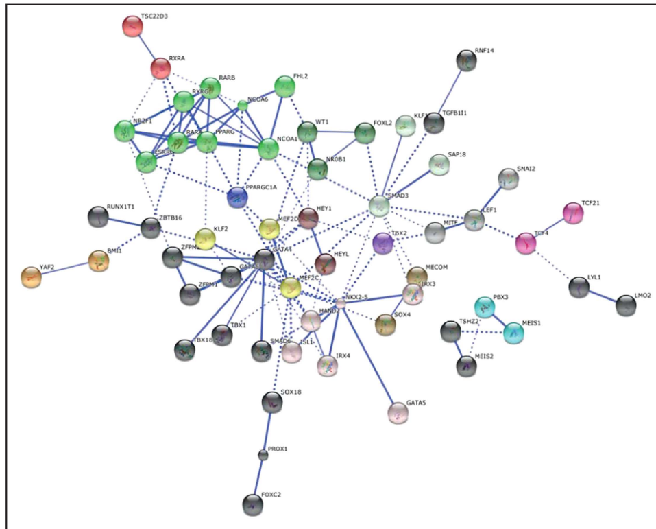
Figure 7. Merged protein-protein interaction network of the enriched transcription factors from all timepoints (d5, d7, d10, d14), obtained from STRING. Interactions with a high confidence > 0.7 are visualized. Proteins are clustered using the MCL algorithm. Every color represents a cluster. Inter-cluster edges are represented by dashed lines. Non-connected gene nodes are not visualized. We could identify the development of three distinct large node clusters, including retinoic acid nuclear receptors, containing PPAR \gamma and RAR \alpha/\beta , and two large interconnected cardiac networks centered on either GATA4 or NKX-5.
