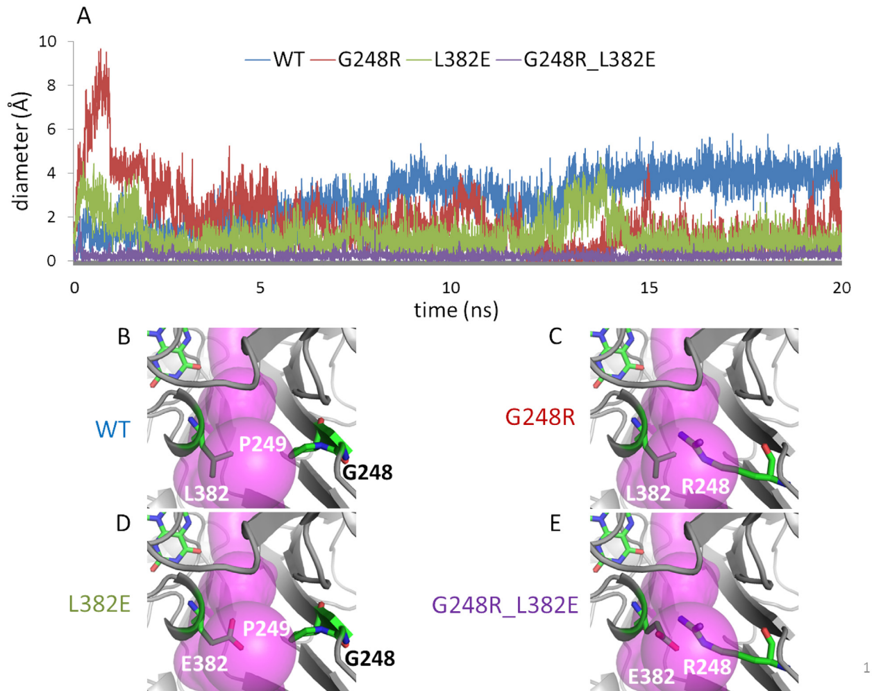
Fig 9. Molecular dynamics of Coq6p homology models. A): Time-evolution of substrate access channel diameter at choke points over MD runs for Coq6p_MODELLER homology model: wild-type (blue trace), Coq6p-G248R (red trace) and Coq6p-L382E (green trace) single mutants, and the Coq6p-G248R-L382E double mutant (purple trace). B): In the wild-type, the channel diameter is large and is constitutively open. C-D): The single mutants display consistently reduced channel diameters which show thermal fluctuations around open and closed states. E): The double mutant displays a channel diameter that is always below the minimum required for substrate binding. In this figure, re face tunnel 1 (purple volume) is oriented directly to the viewer. The pair of residues tracked of the MD calculations as bottlenecks of the channel are represented in sticks.
