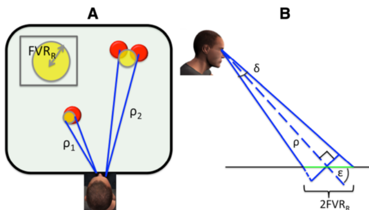
Fig. 3 The visual foveal radius increases as a function of \rho , which implies that, at larger distances, participants can foveate and discriminate multiple objects simultaneously. a Since \rho_2 > \rho_1 , the FVR (also see inset) for \rho_2 is larger. If the participant places the center of the foveal circle strategically during visual search, multiple objects (red circles) could be foveated simultaneously. b Schematic diagram of how the FVR is computed from the eye tracking data
