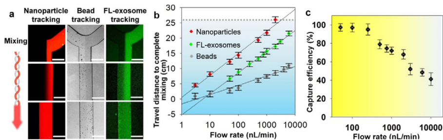
Fig. 2. Microfluidic continuous-flow mixing for efficient exosome isolation. (a) Two-stream particle mixing in the microchannel. Left: Fluorescence CCD images of mixing process for a stream of Texas Red labeled nanoparticles (50 nm) co-flowed with a bead solution. Middle: Immuno-magnetic beads (2.8 \mu\text{m} ) tracked under bright field for mixing with human blood plasma. Right: Mixing of fluorescently labeled exosomes with antibody beads. Exosomes were purified from ovarian cancer patient plasma by ultracentrifugation. Scale bars: 300 \mu\text{m} . (b) Plots of minimum travel length required for uniform mixing over a flow rate range. Grey dashed line indicates mixing channel length in the ExoSearch chip. (c) Exosome capture efficiency as a function of mixing flow rate measured using purified, fluorescently labeled exosomes and capture beads.
