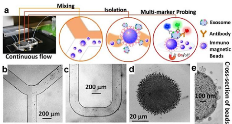
Fig. 1. (a) Workflow of the ExoSearch chip for continuous mixing, isolation and in-situ, multiplexed detection of circulating exosomes. (b) – (c) Bright-field microscope images of immunomagnetic beads manipulated in microfluidic channel for mixing and isolation of exosomes. (d) Exosome-bound immunomagnetic beads aggregated in a microchamber with on/off switchable magnet for continuous collection and release of exosomes. (e) TEM image of exosome-bound immunomagnetic bead in a cross-sectional view.
