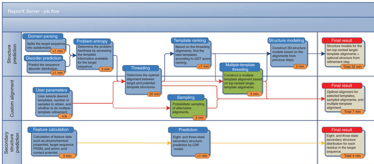
Figure 2. Workflow used by the RaptorX server. Outline of the three modeling tasks users can accomplish using the RaptorX server, namely tertiary structure prediction, custom alignment and secondary structure prediction. For each stage, details of the computation and approximate completion time for a 250-residue target sequence are given (for threading; the indicated time is for a full template library scan). Blue boxes indicate mandatory stages, green boxes indicate optional stages and gray boxes indicate the resulting output. The blue, red and yellow directed paths indicate the flow for structure prediction, custom alignment jobs and secondary structure prediction, respectively. Dashed and solid paths indicate that the subsequent steps are optional and required, respectively. n/a, not applicable.
