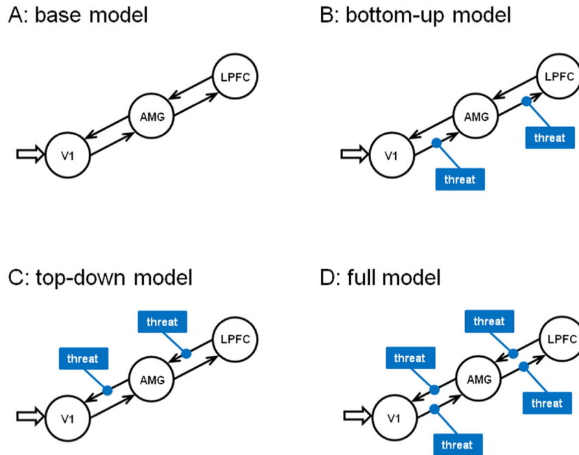
Fig. 2. Model specification. A, Basic structure of the three-area model: visual stimulus presentation drives V1 activity, which is bidirectionally connected to AMG, which in turn is bidirectionally connected to the LPFC. B, Bottom-up model: the modulatory effect of threat is only mediated via bottom-up connections from V1 to AMG to LPFC. C, Top-down model: the modulatory effect of threat is only mediated via top-down connections from LPFC to AMG to V1. D, Full model: the modulatory effect of threat is mediated via both bottom-up and top-down connections between V1 and AMG, and between AMG and LPFC.
