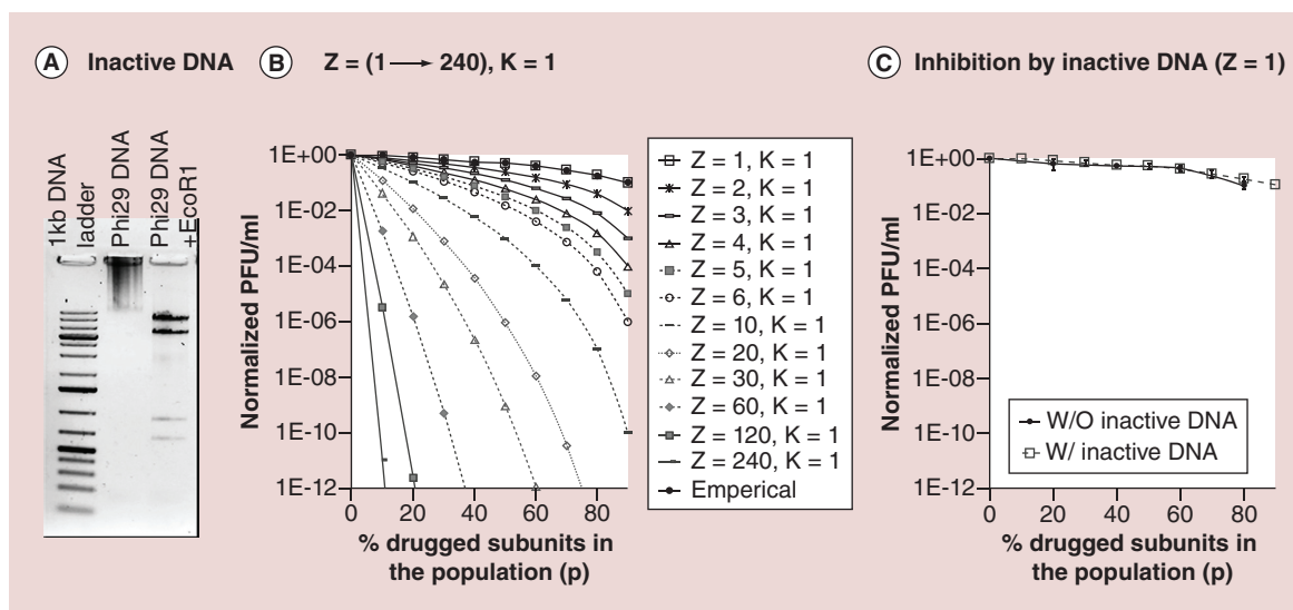
Figure 2. Theoretical plot (with variable Z) and empirical data to illustrate inhibition efficiency with drug targeting to genomic DNA (Z=1). (A) Gel showing the phi29 genome DNA treated with endonuclease EcoRI. (B) Plot of virion assembly derived from binomial distribution Equation 2, which showed that the DNA has stoichiometry of 1. (C) Viral assembly inhibition effect of mutant DNA as model of drugged component with Z = 1, showing the linear relationship to p with low slope.
