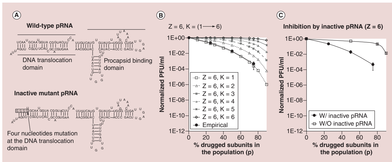
Figure 3. Theoretical plot (K = 1 to 6) and empirical data to illustrate inhibition efficiency with drug targeting pRNA (Z = 6). (A) The sequence and secondary structure of wild-type pRNA of phi29 DNA packaging motor (upper panel) and inactive mutant pRNA with four bases mutation at 5' end of the DNA translocation domain serving as a model of drugged inactive pRNA (lower panel). (B) Fitting the phage assembly inhibition result by inactive mutant pRNA with the theoretical plots derived from Equation 2 matched with Z = 6 and K = 1. (C) Comparing the viral assembly inhibition effect by drugged pRNA at different concentration with the undrugged pRNA with same dilution factor. W: With; W/O: Without.
