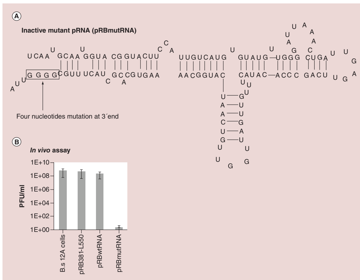
Figure 4. Complete inhibition of viral assembly in vivo by mutant pRNA as a model of drugged complex ( Z = 6 ). (A) Inactivation of pRNA by introducing a 4-nucleotide mutation at the 3' end. (B) Virion production by wild-type phi29 infection using host cell B. subtilis harboring plasmid expressing mutant pRNA, wild-type pRNA or plasmid only.
