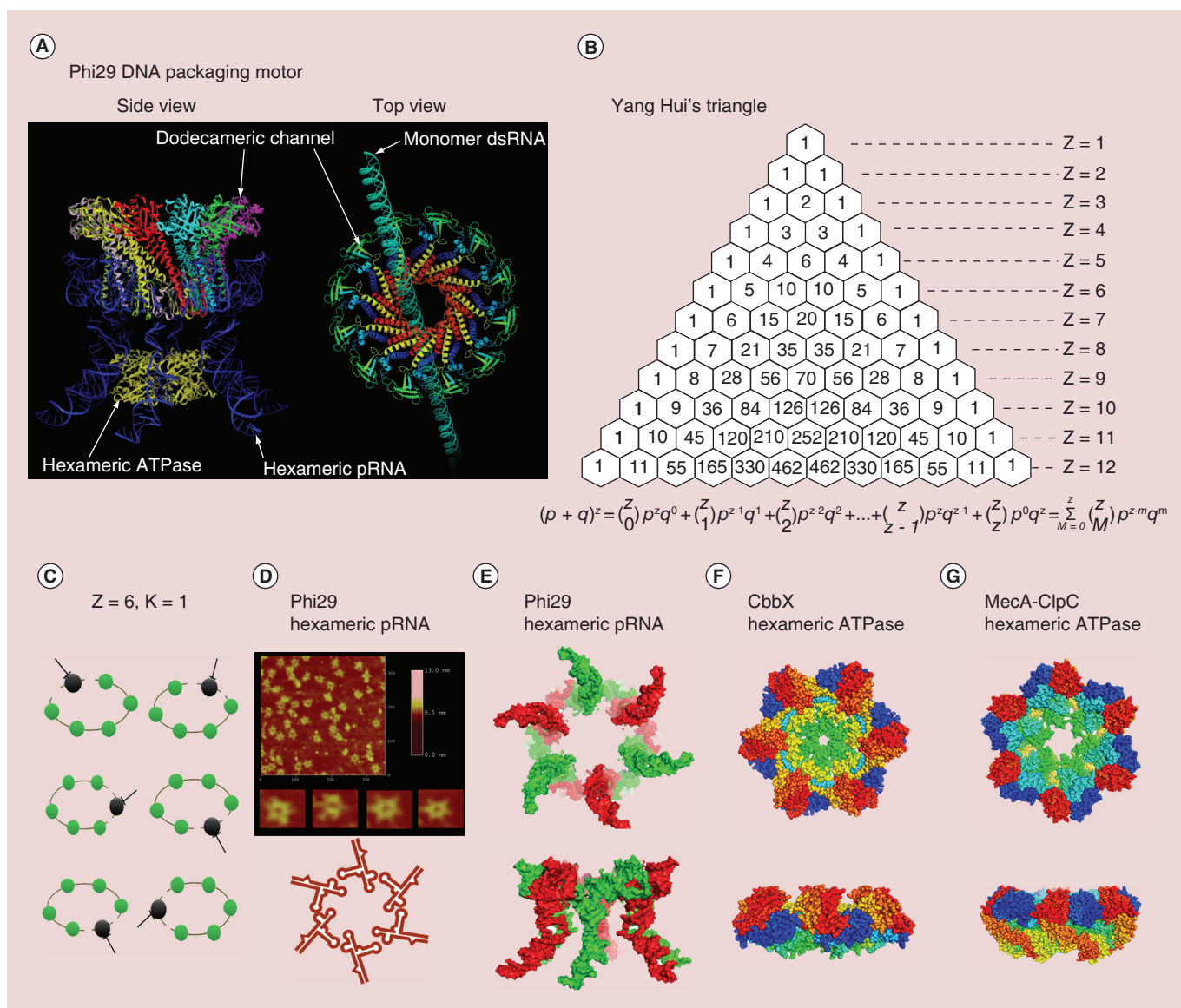
Figure 1. Stoichiometry of viral DNA packaging motor. (A) Illustration of Phi29 DNA packaging motor composed of one copy of genomic DNA that revolves through the channel wall (left panel), six copies of pRNA, six copies of ATPase gp16 and a connector channel. (B) Yang Hui Triangle. (C) Illustration of Z = 6 and K = 1, drug targeting anyone subunit of the complex will block its activity. (D) Atomic force microscopy image of hexameric re-engineered pRNA rings. (E) 3D structure of hexameric pRNA ring top view and side view from the crystal structure of 3WJ (PDB ID: pRNA 3WJ, 4KZ2). (F) A crystal hexameric structure of AAA+ Protein CbbX with top view and side view [59] (PDB ID: CbbX, 3Zuh[60]). (G) Structure of the hexameric AAA+ molecular machine ClpC with adaptor protein MecA [61] (PDB ID: MecA-ClpC, 3PXG). AAA+: ATPases associated with diverse cellular activities.
