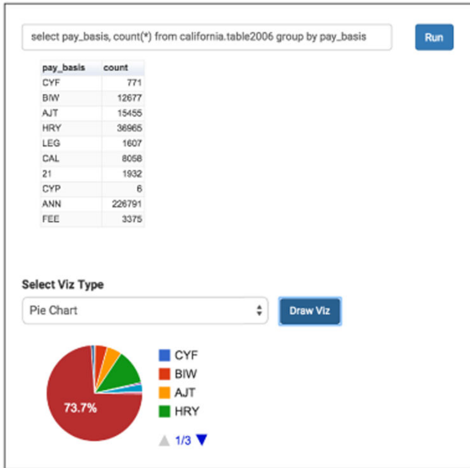
Figure 3. A screenshot of the visualization app (DViz)
