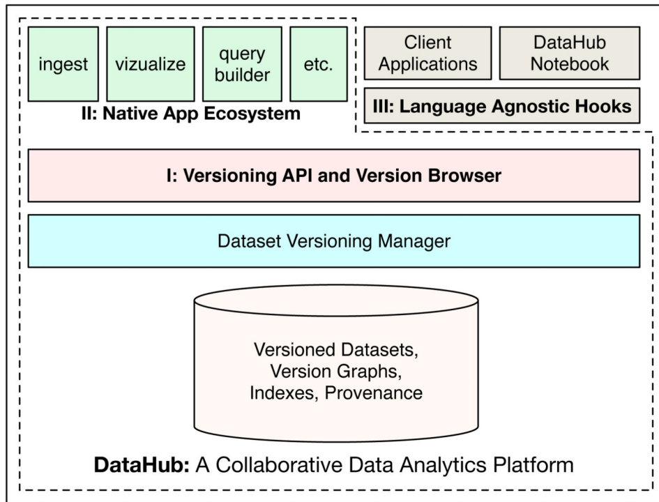
Figure 1. DataHub Architecture
