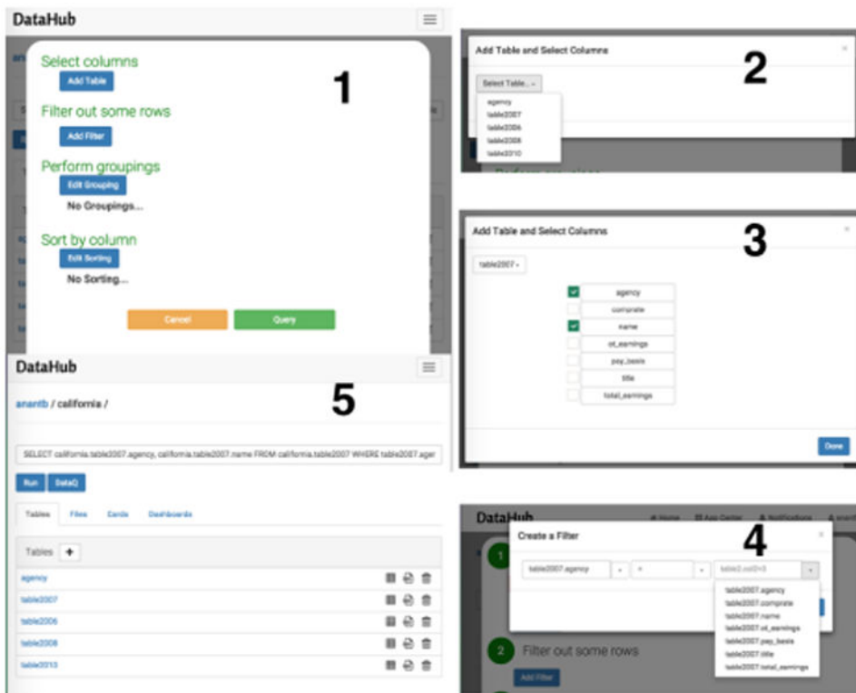
Figure 4. A screenshot of query builder app (DataQ)
