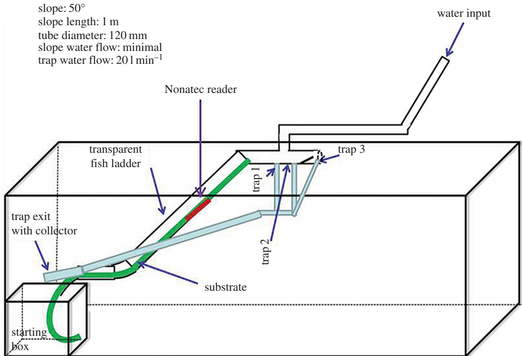
Figure 2. Schematic representation of the experimental fishway device.
