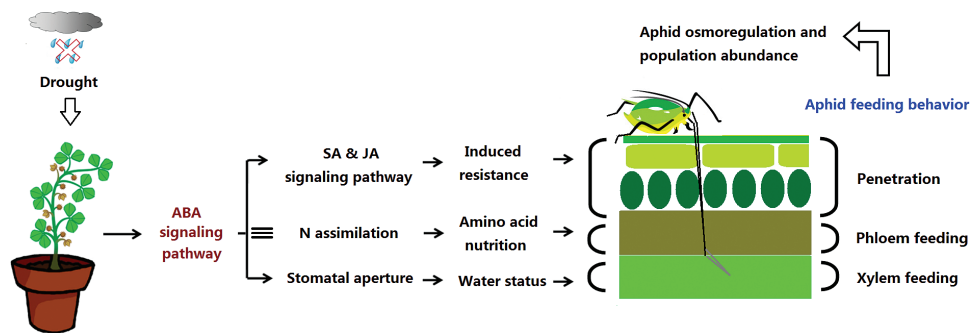
Fig. 9. A model summarizing the effects of the up-regulated ABA signaling pathway on aphid feeding in the M. truncatula -pea aphid system under drought stress. ≡ indicates that drought-induced up-regulation of the ABA signaling pathway did not affect the N nutrition of plants.
