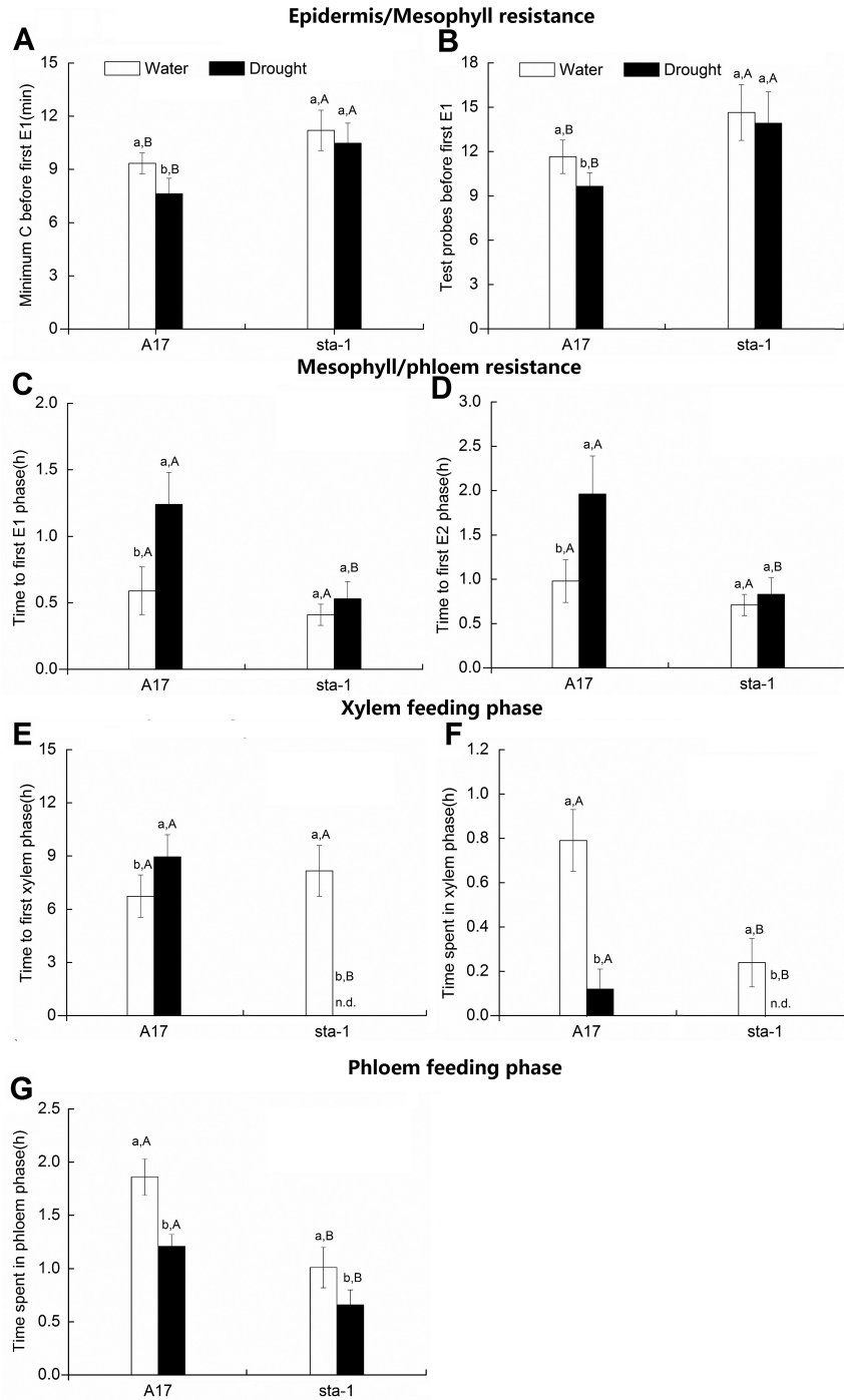
Fig. 2. Electrical penetration graph (EPG) results for pea aphids feeding for 12h on A17 and the sta-1 mutant plants grown under well-watered (water) or drought conditions. (A) Minimum C before first E1; (B) number of probes <3min before first E1; (C) time to first E1; (D) time to first E2; (E) time to first G phase; (F) time spent in the xylem phase; and (G) time spent in the phloem phase. Each value is the mean ( \pm SE) of 24 biological replicates. Different lower case letters indicate significant differences between water treatments within the same genotype. Different upper case letters indicate significant differences between genotypes within the same water treatment as determined by Tukey's multiple range test at P < 0.05 .
