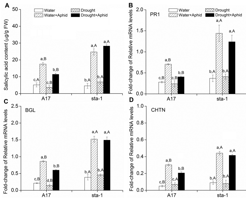
Fig. 4. SA content and expression of genes involved in the SA signaling pathway in two Medicago truncatula genotypes grown under well-watered or drought conditions with and without pea aphid infestation. (a) SA content; (b) pathogenesis-related protein ( PR ); (c) \beta -1,3-glucanase ( BGL ); and (d) endochitinase ( CHTN ) expression. Each value is the mean ( \pm SE) of eight replicates. Different lower case letters indicate significant differences among the combinations of aphid treatment and water treatment within the same genotype. Different upper case letters indicate significant differences between genotypes within the same water treatment and aphid treatment as determined by Tukey's multiple range test at P < 0.05 .
