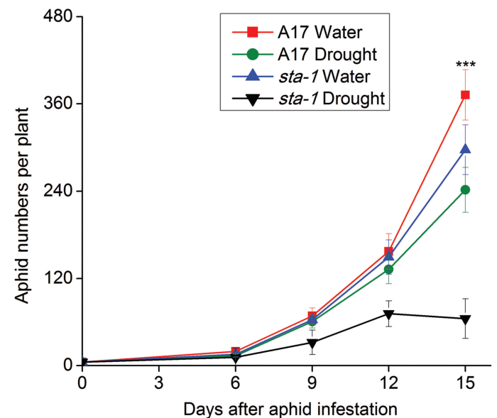
Fig. 1. Numbers of pea aphids per plant when fed on wild-type A17 and sta-1 (sensitivity-to-ABA) mutant plants grown under well-watered (water) and drought-stressed (drought) conditions. Each value is the mean ( \pm SE) of 12 replicates. Significant differences at P < 0.05 are indicated by asterisks. (This figure is available at JXB online.)
