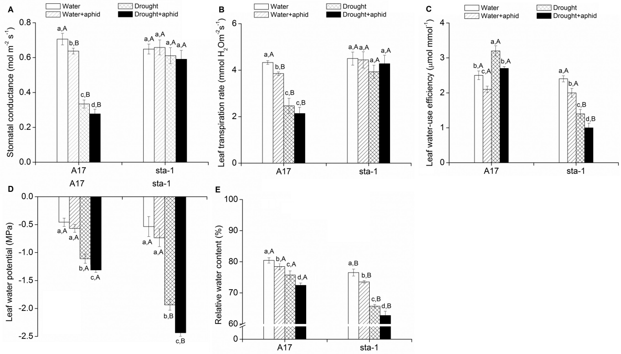
Fig. 7. Gas exchange parameters and water status in two Medicago truncatula genotypes grown under well-watered and drought conditions with and without pea aphid infestation. (A) Stomatal conductance; (B) transpiration rate; (C) water-use efficiency (D) water potential; and (E) relative water content. Each value represents the mean ( \pm SE) of eight replicates. Different lower case letters indicate significant differences among the combinations of aphid treatment and water treatment within the same genotype. Different upper case letters indicate significant differences between genotypes within the same water treatment and aphid treatment as determined by Tukey's multiple range test at P < 0.05 .
