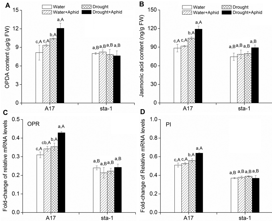
Fig. 5. Key metabolites and relative expression of key genes involved in the JA signaling pathway for two M. truncatula genotypes grown under well-watered or drought conditions with and without pea aphid infestation. (A) (+)-12-oxophytodienoic acid (OPDA) content; (b) JA content; (c) 12-OPDA reductase ( OPR ) expression; and (d) cysteine proteinase inhibitor ( PI ) expression. Each value represents the mean ( \pm SE) of eight replicates. Different lower case letters indicate significant differences among the combinations of aphid treatment and water treatment within the same genotype. Different upper case letters indicate significant differences between genotypes within the same water treatment and aphid treatment as determined by Tukey's multiple range test at P < 0.05 .
