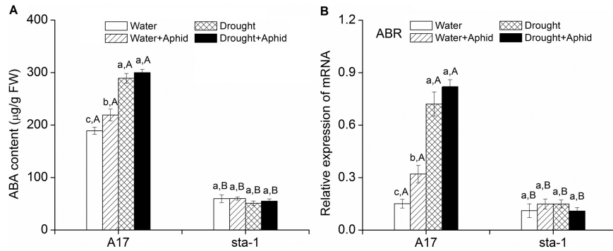
Fig. 3. ABA content and relative expression of the downstream ABA-responsive protein gene ( ABR ) for two M. truncatula genotypes grown under well-watered (water) or drought conditions with and without pea aphid infestation. Each value represents the mean ( \pm SE) of four replicates. Different lower case letters indicate significant differences among the combinations of aphid treatment and water treatment within the same genotype. Different upper case letters indicate significant differences between genotypes within the same water treatment and aphid treatment as determined by Tukey's multiple range test at P < 0.05 .
