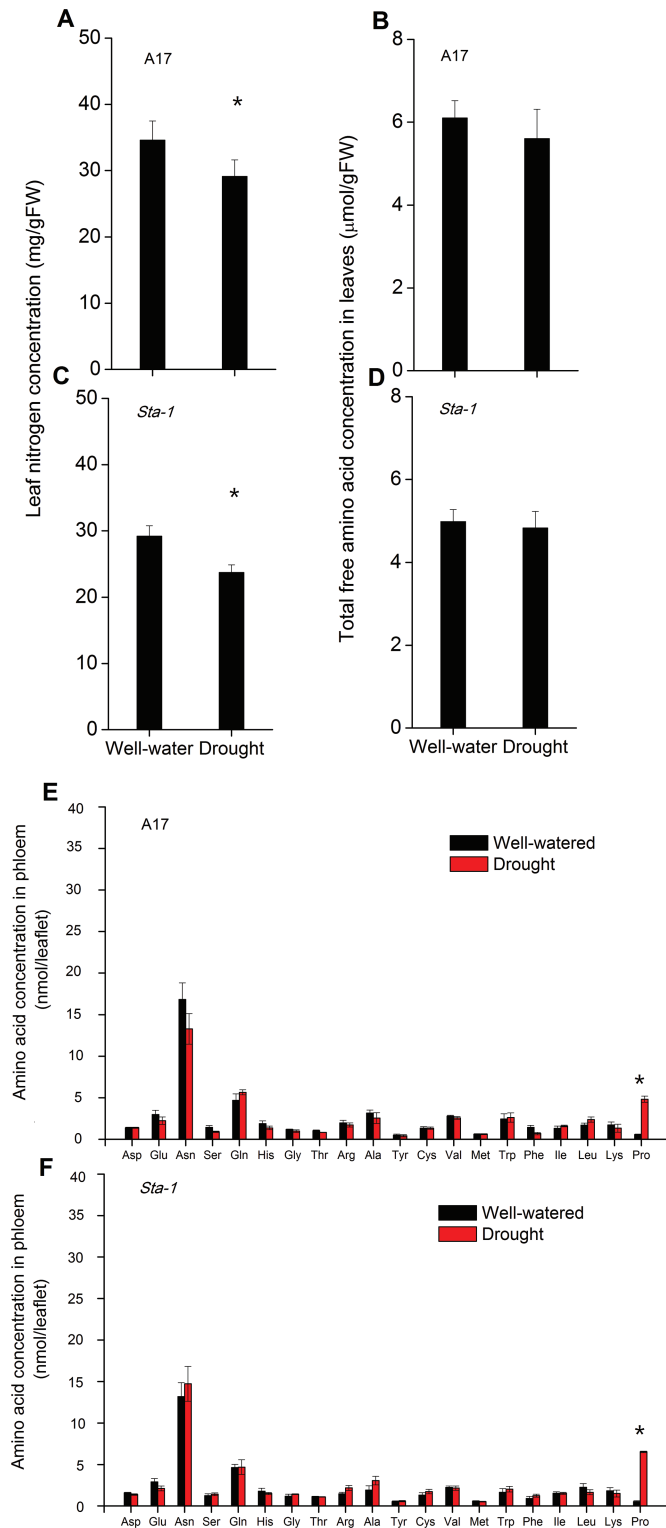
Fig. 6. N concentration and phloem amino acid concentration for two M. truncatula genotypes grown under well-watered or drought conditions without pea aphid infestation. Significant differences at P < 0.05 are indicated by asterisks.
