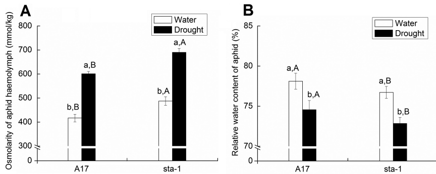
Fig. 8. Hemolymph osmolarity and relative water content of pea aphids when fed on wild-type A17 and the sta-1 (sensitivity-to-ABA) mutant plants grown under well-watered (water) and drought stress conditions. (A) Hemolymph osmolarity; (B) relative water content. Different lower case letters indicate significant differences between water treatments within the same genotype. Different upper case letters indicate significant differences between genotypes within the same water treatment as determined by Tukey's multiple range test at P < 0.05 .
