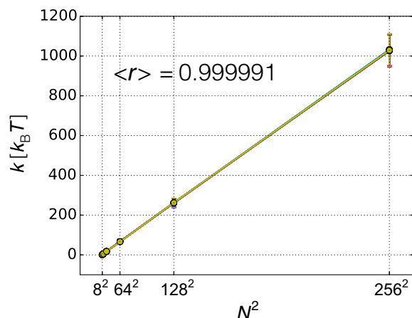
Fig. 3. Scaling of the metaference harmonic restraint intensity in the absence of noise in the data. We verified numerically that in the absence of noise in the data and with a Gaussian noise model, the intensity of the metaference harmonic restraint k = \sum_{r=1}^N \frac{1}{\sigma_r^2} , which couples the average of the forward model over the N replicas to the experimental data point (Eq. 7), scales as N^2 . This test was carried out in the model system at five discrete states, with 20 data points and with the prior at 16% accuracy. For each of the 20 data points, we report the average restraint intensity over the entire Monte Carlo simulation and its SD when using 8, 16, 32, 64, 128, and 256 replicas. The average Pearson's correlation coefficient on the 20 data points is 0.999991 \pm 3 \times 10^{-6} , showing that metaference coincides with the replica-averaging maximum entropy modeling in the limit of the absence of noise in the data.
