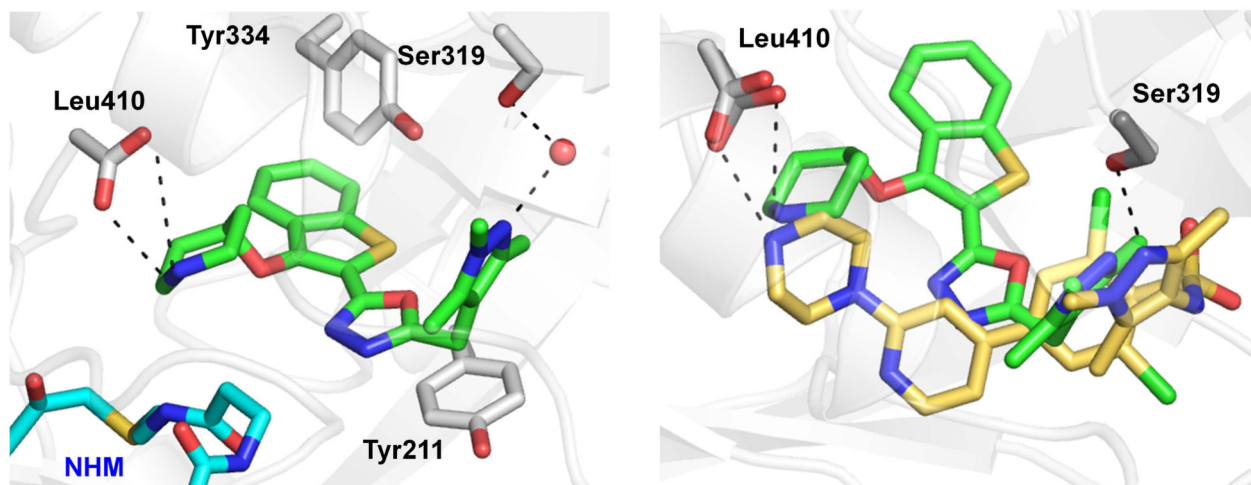
Figure 4. Compounds 1a-c and 2a-b bind in the Plasmodium NMT peptide binding pocket and inhibit the recombinant enzyme
