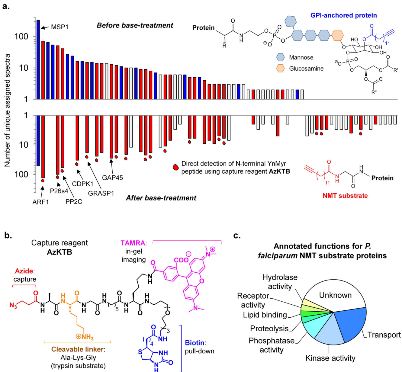
Figure 3. Chemical proteomic discovery and direct detection of modification site for N -myristoylated and GPI-anchored proteins in blood stage P. falciparum
