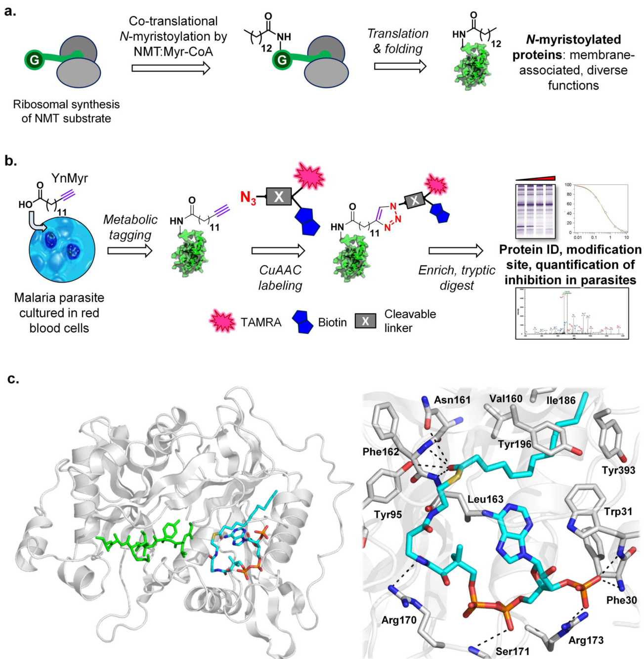
Figure 1. YnMyr-CoA is an effective substrate mimic for P. falciparum and P. vivax N -myristoyltransferases
