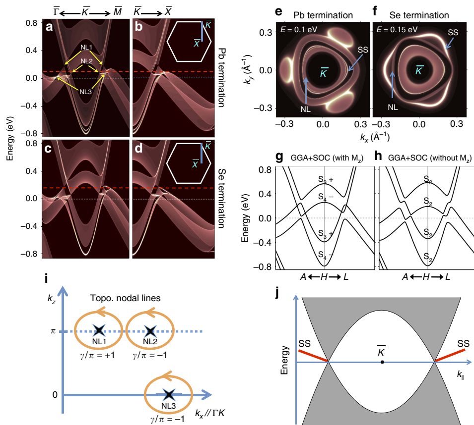
Figure 5 | Topological-nodal rings and associated surface states. (a,b) DFT project bulk bands and surface bands (bright white lines) of Pb-terminated (001) surface along \bar{\Gamma} - \bar{K} - \bar{M} and a generic direction \bar{K} - \bar{X} , respectively. (c,d) Same as a,b but of Se-terminated (001) surface. (e,f) The isoenergy contour showing the nodal-line states (NL) and surface states (SS). The energy is 0.10 and 0.15 eV above the Fermi level for Pb- and Se termination, respectively, as indicated by the red dashed lines in a-d. (g,h) Bulk band structure of PbTaSe 2 with and without the reflection symmetry, respectively. In h, the reflection symmetry is broken by moving the Pb atom slightly in the vertical direction. (i) Schematic of the closed contours encircling the nodal lines for the calculation of the winding number. The arrows indicate the direction on the loops along which the Berry's connection is integrated. (j) Schematic of a spectral cut passing \bar{K} . The grey shaded region indicates the projected bulk band associated with a single nodal ring encircling \bar{K} , and the red curves depict the surface states (SS).
