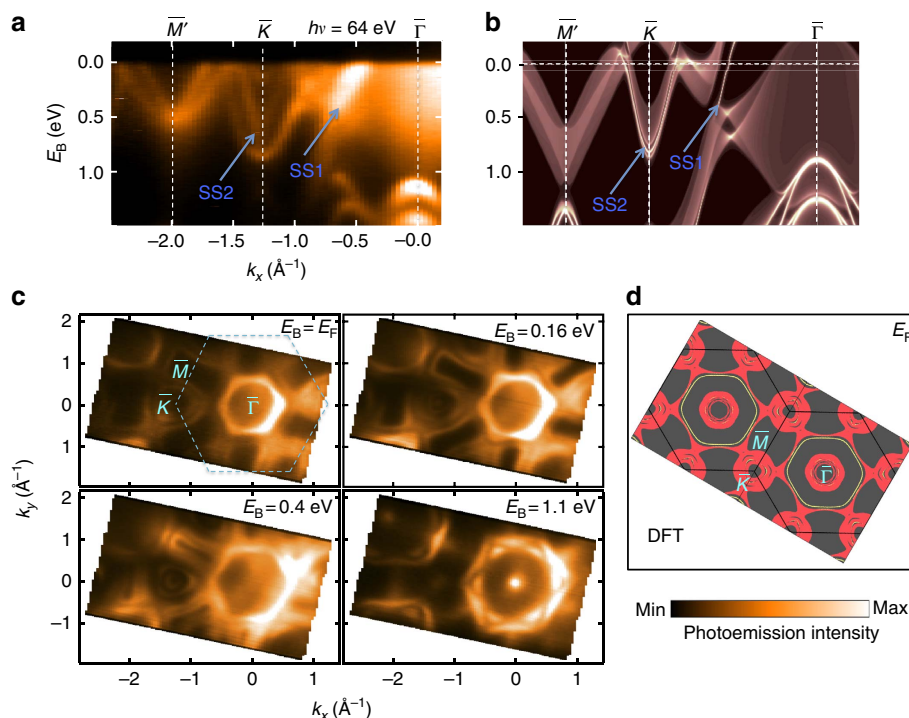
Figure 3 | ARPES mapping and band calculation of PbTaSe 2 . (a) ARPES spectra taken along \bar{M} - \bar{K} - \bar{\Gamma} with 64-eV photons. (b) DFT-projected bulk bands and surface bands (bright white lines) of (001) surface with Pb termination. (c) ARPES isoenergy contours taken with 64-eV photons. (d) DFT Fermi surface contour of PbTaSe 2 (001) surface. The yellow lines indicate the surface states on Pb-terminated (001) surface.
